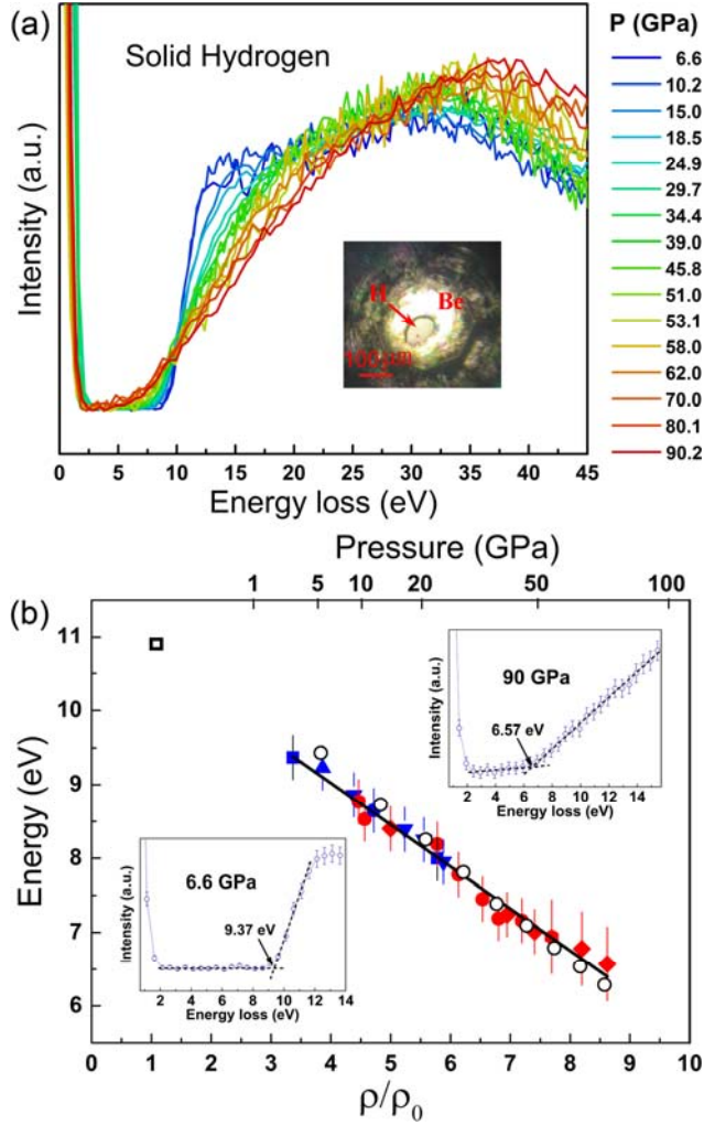
Fig. 3 (a) IXS spectra of solid hydrogen at high pressures from 6.6 to 90.2 GPa. The inset photomicrograph shows the 100 \mu\text{m} hydrogen sample at 90.2 GPa. (b) The band gap of solid hydrogen determined at the breaking points of the slopes of the IXS spectra (illustrated in the insets); blue, experiments at APS; red, experiments at SSRF; seven different solid symbols represent separate DAC IXS experiments; open square, the zero pressure ( <10^{-7} torr), low temperature (2 K) threshold energy from Ref. [11]; open circles, theoretical calculations; solid line, linear regression of the IXS experimental data.
