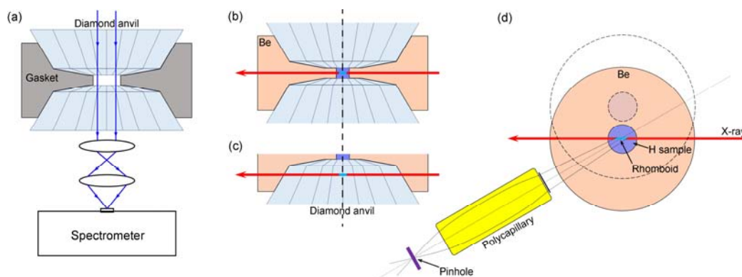
Fig. 1. Schematic drawings showing typical (a) optical and (b-d) IXS geometries using a DAC; (a-c) side view and (d) top view are not drawn to scale. The red lines in (b) and (d) show the narrowly focussed incident x-ray beam passing through the blue hydrogen sample while avoid the diamond anvils on top and bottom (b), and gasket on the side (d). (c), the diamond anvil was moved 100 \mu\text{m} vertically to collect signal from the diamond background and (d) the dotted line shows the DAC was moved 150 \mu\text{m} sideways to collect the Be gasket background. An x-ray confocal “polycapillary” device is used to select the signal coming from the rhomboid-shaped (light blue colored) portion of the hydrogen sample.
