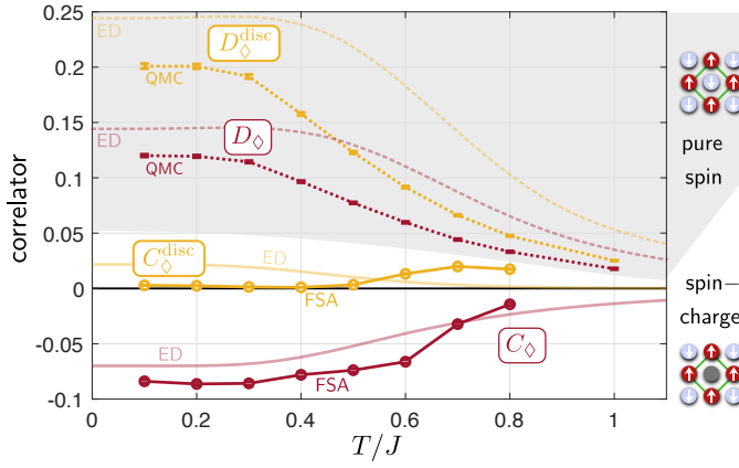
FIG. 4. Temperature dependence of the higher-order correlations C_\Diamond (red) and the disconnected C_\Diamond^{\text{disc}} (yellow) parts (using Eq. (2)). We compare the corresponding correlators D_\Diamond in the undoped Heisenberg model (top) to predictions for a mobile dopant (with t/J = 2 ), using the FSA in a 16 \times 16 lattice based on Heisenberg quantum Monte Carlo (QMC) snapshots, and ED simulations in a periodic 4 \times 4 system.
