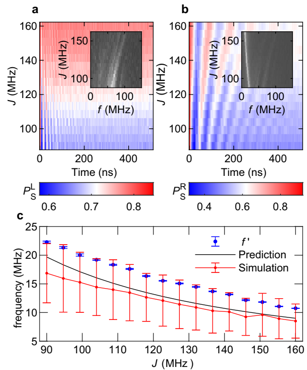
FIG. 2. Four-spin dynamics vs. J with the chain initialized as a singlet. (a) Left-pair singlet return probability P_S^L vs. J and evolution time showing the dynamics of the chain. Inset: absolute value of the fast Fourier transform of the data. (b) Right-pair singlet return probability P_S^R vs. J and interaction time demonstrating spin-state oscillations between end spins. Inset: absolute value of the fast Fourier transform of the data. f indicates frequency. (c) Extracted end-spin oscillation frequency f' vs. J . f' is the fitted frequency of the end-spin oscillations in (b) and corresponds to the peak frequencies in the inset of (b). Theoretical predictions generated from Equation 2 and from numerical simulations are also shown. The error bars associated with the data are the standard errors of the fitted frequencies corresponding to each horizontal line in (b). The error bars associated with the simulation are the standard deviations of Monte-Carlo simulations of the superexchange frequency [29]. These error bars illustrate the expected size of systematic errors associated with calibration of the exchange couplings.
