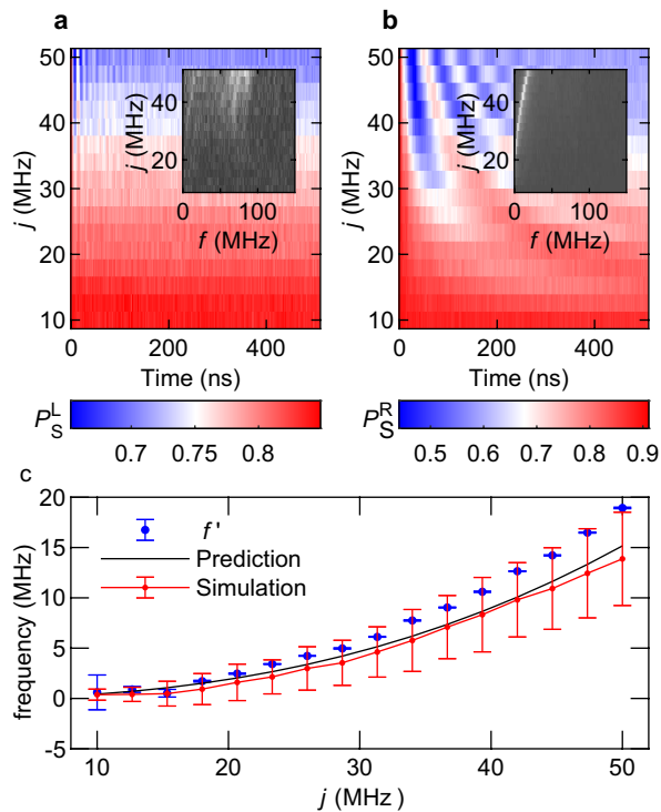
FIG. 3. Four-spin dynamics vs. j with the chain initialized as a singlet. (a) Left-pair singlet return probability P_S^L vs j and evolution time showing the dynamics of the chain. Inset: absolute value of the fast Fourier transform of the data. (b) Right-pair singlet return probability P_S^R vs. j and interaction time demonstrating end-spin oscillations. Inset: absolute value of the fast Fourier transform of the data. f indicates frequency. (c) Extracted end-spin oscillation frequency f' vs. j . f' is the fitted frequency of the end-spin oscillations in (b) and corresponds to the peak frequencies in the inset of (b). Theoretical predictions generated from Equation 2 and from numerical simulations are also shown. The error bars are computed as discussed above.
