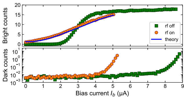
FIG. 2. Impact of trap rf on SNSPD performance. We plot bright (top) and dark (bottom, log scale) counts in a 200 \mu s detection window versus SNSPD bias current, with trap rf either off (green squares) or on (orange circles), using laser scatter to simulate ion fluorescence for the bright counts. The blue line is a fit to a theoretical model accounting for induced rf currents in the SNSPD. The bright counts are background-corrected by subtracting the measured dark counts at each bias current. The 68 % confidence intervals on the reported values are smaller than the plot symbols.
