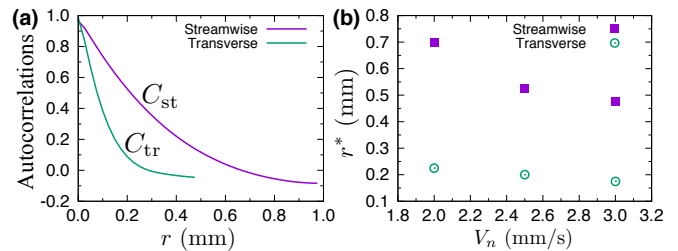
FIG. 4. (a) Autocorrelations as a function of distance r at V_n = 2.5 mm/s. (b) Distances r^* where the autocorrelations decays to 0.1.
