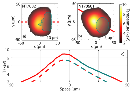
FIG. 2. a-b) Profiles of hot spot temperature for experiments N170821 and N170601 conducted with a 10 \mu\text{m} and 5 \mu\text{m} fill tube, respectively. The shaded region indicates the region of fill tube mix. The dashed and solid lines indicate the direction along which the temperature profile in c) are taken. The over-plotted dashed and solid green lines denote the location of the mixed material.
