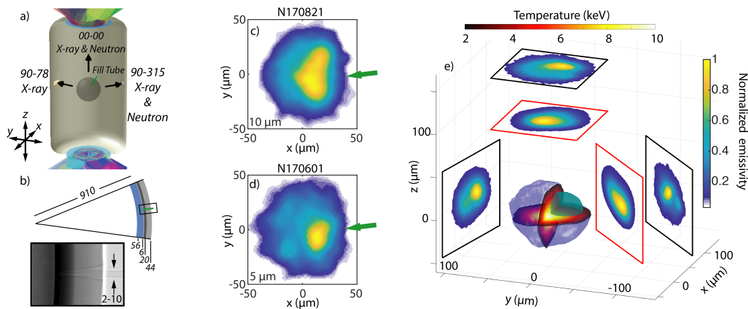
FIG. 1. a) Experimental setup showing the hohlraum and capsule target. X-ray and neutron images are taken along 3 and 2 lines of sight, respectively[17, 18]. The polar and azimuthal angle for each detector are denoted. The fill tube enters the capsule at an angle of 90-07 as indicated by the green line. b) Illustration and radiograph of the initial capsule with dimensions given in \mu\text{m} . The light and dark gray regions denote the undoped, doped with an atomic fraction of 0.33% of tungsten layers of the HDC ablator, respectively. The blue region denotes the DT ice layer. c-d) Observed x-ray emission along the 00-00 line of sight at stagnation integrated over \sim 125 ps for experiments conducted with a 10 and 5 \mu\text{m} fill tube, respectively. The green arrow indicates the initial orientation of the fill tube. e) 3D reconstruction of the hot spot temperature ( > 2 keV) for N170601 produced using 2 temporally integrated neutron emission measurements (outlined in red). Using 3 x-ray images (outlined in black) the region of localized mix within the hot spot can be reconstructed and is shown by the green contour.
