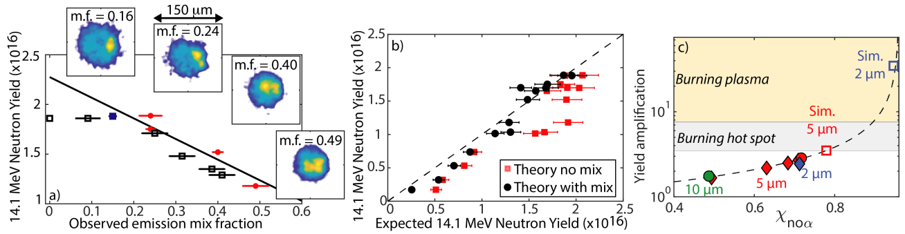
FIG. 3. a) Yield vs. observed emission mix fraction for 5 experiments with same drive conditions. The fill tube diameter was 2 and 5 \mu\text{m} for the blue and red data, respectively. Open black squares are the observed emission mix fractions of simulated x-ray images from implosions with increasing fill tube diameters (0, 2 \mu\text{m} , 5 \mu\text{m} , 10 \mu\text{m} , 15 \mu\text{m} , 20 \mu\text{m} ). The solid line represents the best linear fit to the data. Images of the x-ray emission with energies > 10 keV for the different observed mix fractions are also shown. b) Observed yield vs. expected yield using Eqn. 2, with and without taking into account the impact of radiative loss shown by the black circles and red squares, respectively. c) Inferred yield amplification vs. \chi_{no\alpha} with regions of burning hot spot and plasma denoted as defined by [29]. Green and red circles indicate experiments N170821 and N170601 conducted with a 10 and 5 \mu\text{m} fill tube, respectively. The red and blue diamonds denote experiments shown in Fig 3 a). Higher yield amplifications can be obtained in simulations of implosions of similar adiabat (2.9 vs. 3), without drive asymmetries and with 1.15\times larger capsules that absorb \sim 1.15\times more energy and obtain a velocity 1.09\times larger than experiments reported here.
