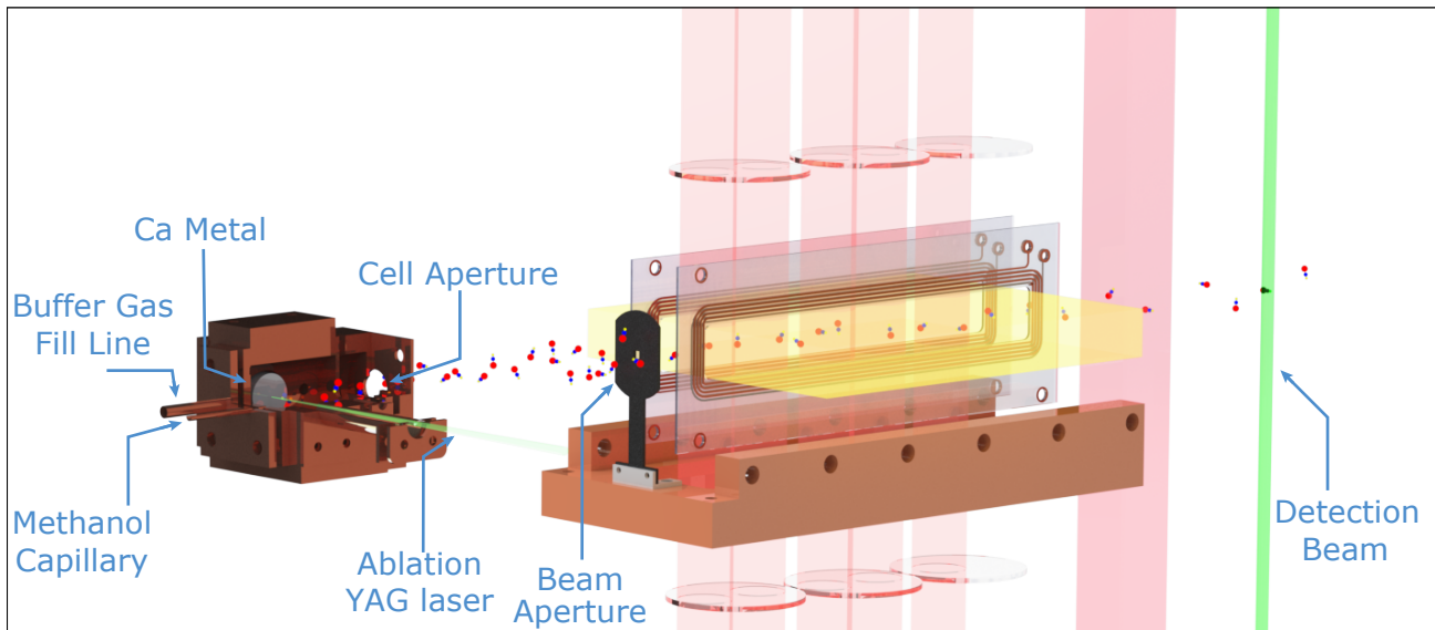
Figure 2. A rendering of the experimental apparatus. On the far left is the two-stage buffer-gas beam source, depicted in cut-away view for clarity. 35.5 cm from the exit of the buffer-gas cell, the molecular beam is collimated by a 3 mm square beam aperture. 39 cm from the cell, the molecules enter the interaction region where they are addressed with light from the main MO cooling beams in the vertical direction. Co-propagating vertically are the (100), (200) and (02 00 ) repumping lasers indicated in red. The (02 20 ) and (01 10 ) repumping light, indicated in yellow, is multipassed in the horizontal direction and extends beyond the MO region. A separate vertically multipassed region containing (100) and (02 00 ) repumping light lies after the magnetic field coils and serves to recover population from excited vibrational states. Finally, the molecules encounter a detection beam of smaller cross-section than the cooling and repumping light, and the resulting laser-induced fluorescence is collected and imaged onto an EMCCD.
