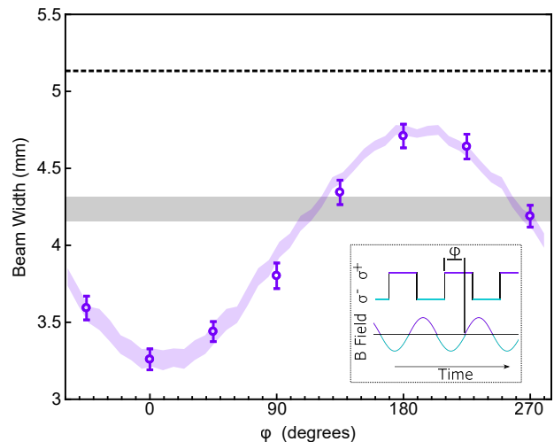
Figure 4. Molecular beam width as a function of phase offset ( \phi ) between the polarization switching of cooling light and the oscillating magnetic field (see inset). The dashed black line indicates the width of the unperturbed beam, the shaded grey region indicates the measured width and associated error of the Doppler cooled beam without an applied magnetic field, and the shaded purple region indicates Monte Carlo simulation results for the full MO configuration. Clear compression at 0 phase corresponds to the MOT configuration, where the laser polarization provides a spatially confining force. At 180 degrees there is expansion of the beam, corresponding to the anti-MOT configuration. The main cooling light is detuned -7 MHz from resonance while all repumping lasers remain resonant. Error bars represent one standard deviation of the fitted Gaussian beam width.
