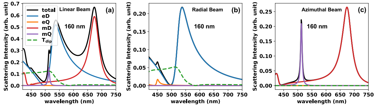
Figure 3: Multipolar decomposition of the scattering spectra. The calculated scattering spectra of single Si nanospheres with diameter 160 for linearly (a), radially (b) and azimuthally (c) polarized beam illuminations. The multi-polar decomposition shows that both electric and magnetic modes are excited for linearly polarized beam; whereas only electric (magnetic) modes are excited for radially (azimuthally) polarized beam illumination. The toroidal dipoles are also excited for linearly and radially polarized beam illuminations.
