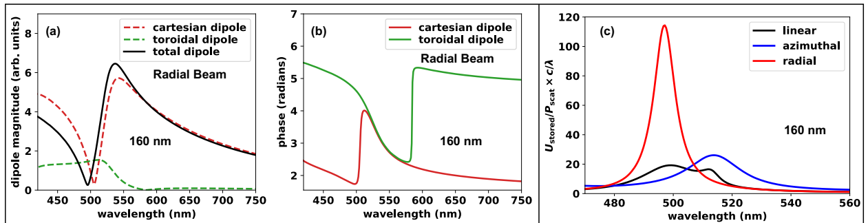
Figure 4: The amplitude (a) and phase (b) of the Cartesian electric and toroidal dipoles under radially polarized beam illumination for d = 160 . The results show that the amplitudes of the Cartesian electric and toroidal dipoles are equal and out-of-phase at \lambda \sim 500 nm for d = 160 nm resulting in excitation of anapole. (c) shows the fraction of the localized vs. radiated energy calculated for linear, radial and azimuthal beam illuminations for d = 160 nm. The stored energy is \sim 6 times greater for radial vs. linear beam illumination.
