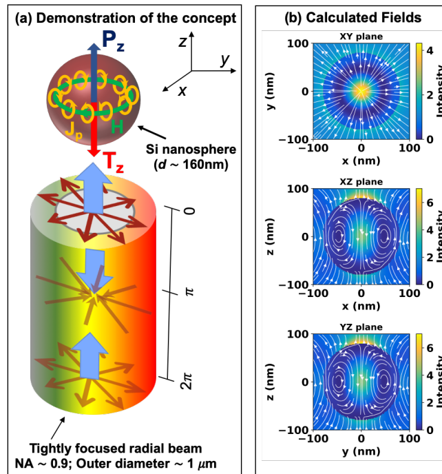
Figure 1: Demonstration of the anapole excitation and simulated electric field distributions. (a) Schematic diagram showing excitation of a Si nanosphere ( d \sim 160 nm) for radially polarized beam excitation. In addition to the z -component of the electric resonances ( P_z ), the radially polarized beam is expected to generate a z -component of the toroidal response ( T_z ) produced by the circulating magnetic field ( H ) associated with the poloidal currents ( J_p ) flowing in the bulk. (b) Streamlines of the total electric field for radially polarized beam illumination as calculated using Generalized Mie Theory show that the toroidal current (given by Eq. 3) is indeed produced within the volume of the nanosphere.
