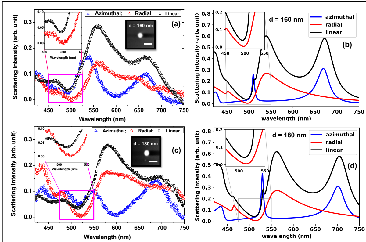
Figure 2: Scattering spectra of single Si nanospheres under linear and vector beam illumination. The experimental (a,c) and simulated (b,d) scattering spectra of single Si nanospheres with diameter 160 (a,b) and 180 nm (c,d), respectively for linearly, radially and azimuthally polarized beam illuminations. The right insets of Figs (a) and (c) show the SEM images of the exact same nanospheres whose scattering spectra are shown. The white scale bars on the SEM images are 500 nm. The results show that the scattering minima are deepest for radial beam excitation at around 500 nm (the regions of interest is shown in the insets) for d = 160 nm (a,b), and at around 520 nm for d = 180 nm (c, d). The simulated spectra were calculated using Generalized Mie Theory over all the scattering angles, whereas the experimental spectra were measured in the backward direction for the angular range determined by the numerical aperture of the microscope objective.
