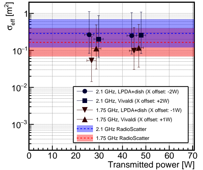
FIG. 4. The effective scattering cross section, \sigma_{\text{eff}} , as a function of transmitter output power, for various receiving antennas (LPDA+dish and Vivaldi) and 2 different frequencies. Errors are statistical and systematic, and dominated by the latter. Each set of 4 points has been clustered around the true X axis value, for clarity, with the offset indicated in the figure legend. The solid bands are \sigma_{\text{eff}} from RadioScatter including statistical and systematic errors.
