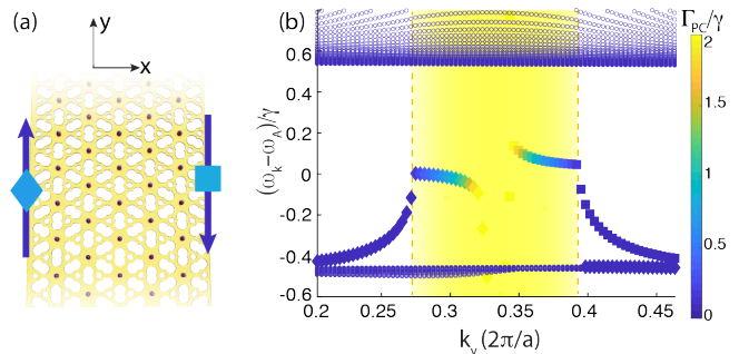
FIG. 4. (a) Infinite stripe of emitters embedded in an extended photonic crystal slab. (b) Edge states inside the band gap near the \mathbf{K} point. Unidirectional edge states on the left (right) boundary are indicated by diamonds (squares). Bulk modes are marked by dots, which form a nearly flat band inside the gap. Yellow shading and yellow dashed lines mark the region where bands can decay into resonant slab modes. Color coding shows the decay rate \Gamma_{\text{PC}} . Relevant parameters are \delta_A = 18.73 \text{ THz} , v_s = 0.25c , |E_0|^2 = 0.1855/a^3 , \Delta = \gamma and \mu B = 0.5\gamma . Results were obtained for a stripe with 81 atoms in the transverse direction. States with 5 times more amplitude on the five leftmost emitter columns than on the five rightmost columns, are classified as edge states.
