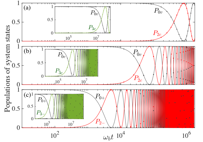
FIG. 2: Super-Rabi oscillations as seen through the population dynamics P_{jk}(t) = |\langle j, k | \psi(t) \rangle|^2 ( j = n, \tilde{n} and k = c, v, +, - ) with n = 2, 3 corresponding to the main and insert parts, respectively. The solid lines and dots correspond to the exact numerical results and the analytical approximate solutions based on \Omega_{\text{eff}}^{(n)} [42], respectively. System parameters are (a) \lambda/\omega_b = 0.03 , \Omega/\omega_b = 0.003 , (b) \lambda/\omega_b = 0.1 , \Omega/\omega_b = 0.003 , (c) \lambda/\omega_b = 0.03 , \Omega/\omega_b = 0.8 , corresponding to the regimes of Figs. 1(b), 1(c) and 1(d), respectively.
