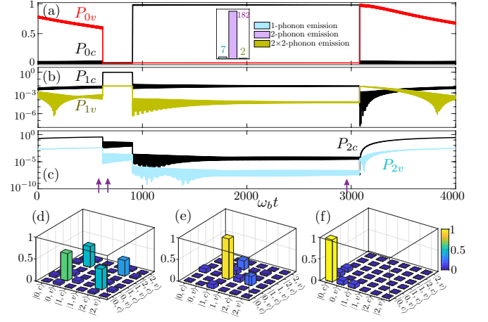
FIG. 4: (a)–(c) Small fraction of a quantum trajectory in the regime of two-phonon emission. The insert bar graphs show the total number of single-, two- and 2n -phonon ( n = 2 ) clicks over 25 quantum trajectories. (d)–(f) Full density matrices of the system at the times indicated with purple arrows in the trajectory, showing the cascade-emission process. System parameters are: \lambda/\omega_b = 0.1 , \Omega/\omega_b = 0.2 , \kappa/\omega_b = 0.002 , \gamma/\omega_b = 0.0002 and \gamma_\phi/\omega_b = 0.0004 , satisfying the regime around sweet point \kappa \approx 10\Omega_{\text{eff}}^{(2)} [42].
