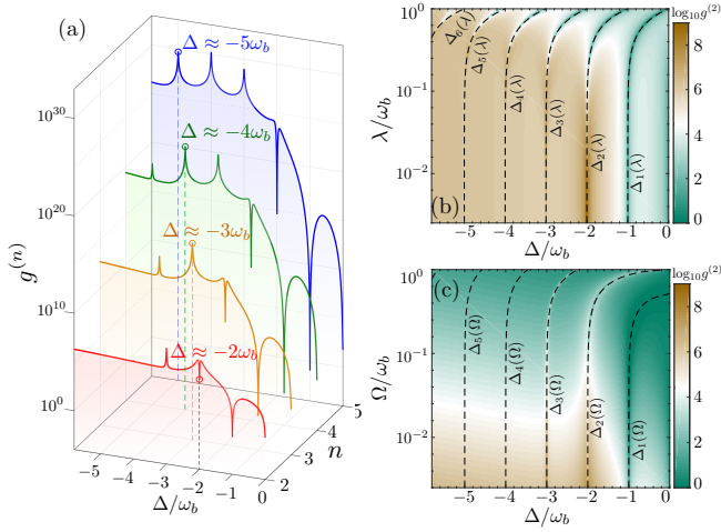
FIG. 3: (a) Equal-time n th-order correlation functions g^{(n)} as a function of \Delta/\omega_b . (b)–(c) Correlation function g^{(2)} for different \lambda/\omega_b (b) and \Omega/\omega_b (c). The dashed lines indicate the n -phonon resonances \Delta = -n\omega_b , \Delta = \Delta_n(\lambda) , and \Delta = \Delta_n(\Omega) . System parameters are (a) \lambda/\omega_b = 0.03 , \Omega/\omega_b = 0.003 , (b) \Omega/\omega_b = 0.003 , (c) \lambda/\omega_b = 0.03 , and \kappa/\omega_b = 0.002 , \gamma/\omega_b = 0.0002 and \gamma_\phi/\omega_b = 0.0004 for panels (a)–(c).
