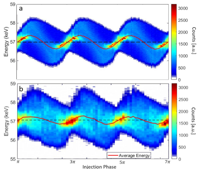
FIG. 2. (a) A two-stage accelerator simulation where the injection phase is linearly varied. e_1 = 58 \text{ MeV/m} . The net energy gain is 350 \text{ eV} , and the peak energy modulation is slightly over 1 \text{ keV} . (b) The measured spectrogram for e_1 = 58 \pm 5 \text{ MeV/m} . The net energy gain is 200 \pm 10 \text{ eV} , and the peak energy modulation is 1.3 \text{ keV} .
