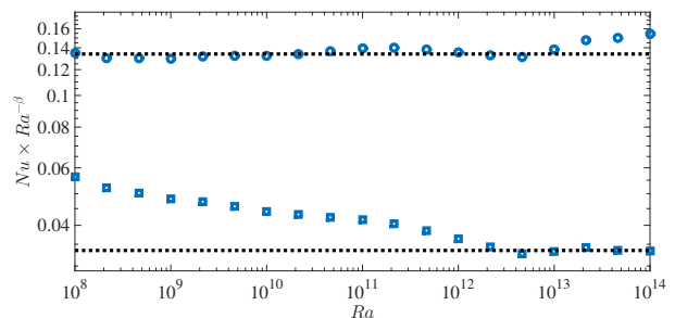
FIG. 1. Compensated plots of Nu \times Ra^{-\beta} vs. Ra . Circles (top) are data of Zhu et al. [1] with \beta = 2/7 while squares (bottom) are the same data with \beta = 1/3 .
