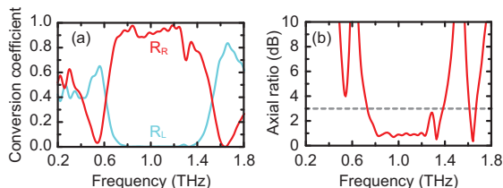
FIG. 3: (a) The retrieved circular polarization states from experimentally measured reflection data when the normally incident THz waves are linearly polarized at 45^{\circ} with respect to the metasurface major principal axis. (b) Axial ratio of the reflected THz waves calculated from experimental measurements.
