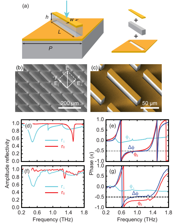
FIG. 2: (a) Schematic of the unit cell of a metasurface structure to realize broadband linear-to-circular polarization conversion. Inset: displacing the metallic structures from the dielectric pillar to reveal the structural details. (b) SEM micrograph of a fabricated metasurface sample, and (c) its false color close-up view. The normally incident THz radiation E is linearly polarized at 45^\circ with respect to the major principal axis. (d) Numerically simulated amplitude reflectivity and (e) phase spectra for the the parallel ( r_{\parallel} and \phi_{\parallel} ) and perpendicular ( r_{\perp} and \phi_{\perp} ) field components, along with their phase difference \Delta\phi . (f) Experimentally measured amplitude reflectivity and (g) phase spectra and their difference.
