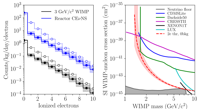
FIG. 4: Left —Projected ionization spectra from a 3 GeV/c 2 WIMP (assuming \sigma_0 = 10^{-41}\text{cm}^2 ) and reactor antineutrino coherent scattering. Projections calibrated by the measurements in this work (solid lines) deviate significantly from those using NESTv2.0 (dashed), which is tuned to fit existing data.
