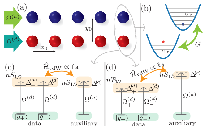
FIG. 1. Schematic of the phonon-swap protocol. (a) For each data atom (red, bottom) we place another auxiliary atom (blue, top) at an equal distance y_0 . We assume a 1D chain of data and auxiliary atoms, with a lattice spacing of x_0 . (b) The Rydberg interactions give rise to effective coupling G between the vibrational modes of the data and auxiliary atoms. (c,d) Two schemes that lead to spin-insensitive interactions between the data and the auxiliary atoms: in (c), the ground states of all atoms are weakly coupled to Rydberg S_{1/2} states. In (d), the data atoms are coupled to n'P_{1/2} states and the auxiliary to nS_{1/2} , where |n - n'| \gg 1 .
