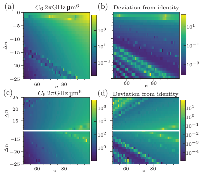
FIG. 3. (a,c) The spin-insensitive interaction strength C_6 and (b,d) deviation from identity for (top) nS_{1/2} + n'S_{1/2} and (bottom) nS_{1/2} + n'P_{1/2} as a function of n and \Delta n = n' - n for Rb atoms. In the case of nS_{1/2} + n'P_{1/2} , we take \min|\Delta n| = 10 .
