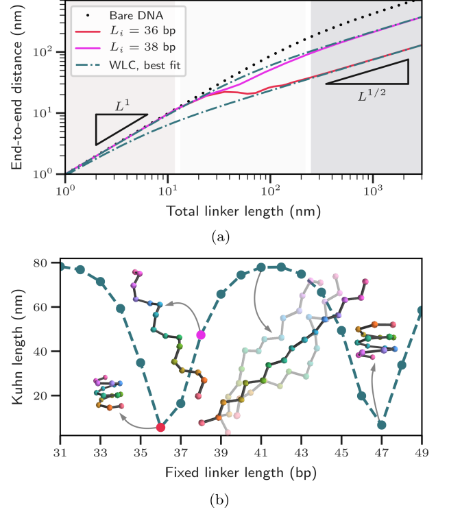
FIG. 2. (a) Average end-to-end distances for homogeneous chromatin chains with 36 bp and 38 bp linkers, compared to bare DNA and the best-fit WLCs. Rigid rod ( L^1 ), Gaussian chain ( L^{1/2} ), and cross-over regimes highlighted. (b) Kuhn lengths of homogeneous chromatin chains are 10.5bp periodic in linker length. Example zero-temperature chain configurations are shown, as well as two Monte Carlo (fluctuating) structures for the 41 bp case. Compact structures (36, 47 bp) have smaller Kuhn lengths than less compact structures (41 bp).
