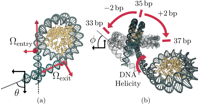
FIG. 1. (a) The structure of a human nucleosome [46] with straight linkers extrapolated from the entry ( \Omega_{\text{entry}} ) and exit ( \Omega_{\text{exit}} ) orientations of the bound DNA. The amount of DNA wrapping the nucleosome dictates the spherical angle \theta . (b) Two adjacent nucleosomes at zero temperature. The DNA double helix has an intrinsic twist density ( \tau = 2\pi/(10.5 \text{ bp}) ), and the binding orientation of the histone octamer must align with the major groove of the double helix. Therefore, as the linker length L connecting two nucleosomes gets longer or shorter, the relative orientations of adjacent octamers change to create an angle \phi = \tau L .
