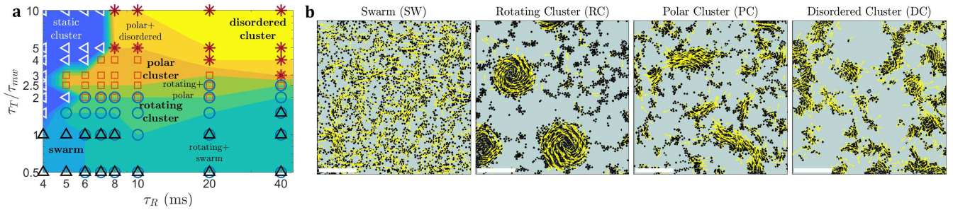
FIG. 3. (a) Collective states formed by Quincke random walkers with different run and turn times ( \tau_R , \tau_T ). Symbols indicate the experimentally observed \triangleleft : static clusters, \Delta : swarm (SW), \circ : rotating clusters (RC), \square : polar clusters (PC), and * : disordered clusters (DC). (b) Snapshots of the SW ( \tau_T/\tau_{mw} = 0.5, \tau_R = 4 ms), RC ( \tau_T/\tau_{mw} = 1.5, \tau_R = 5 ms), PC ( \tau_T/\tau_{mw} = 3, \tau_R = 8 ms) and DC ( \tau_T/\tau_{mw} = 10, \tau_R = 40 ms) phases from the experiments. Scale bar is 1mm. Velocity vectors are superimposed to the particles. Particle area fraction and pulse amplitude are constant in all experiments and are equal to \phi \approx 0.15 and E = 2.08 MV/m, respectively.
