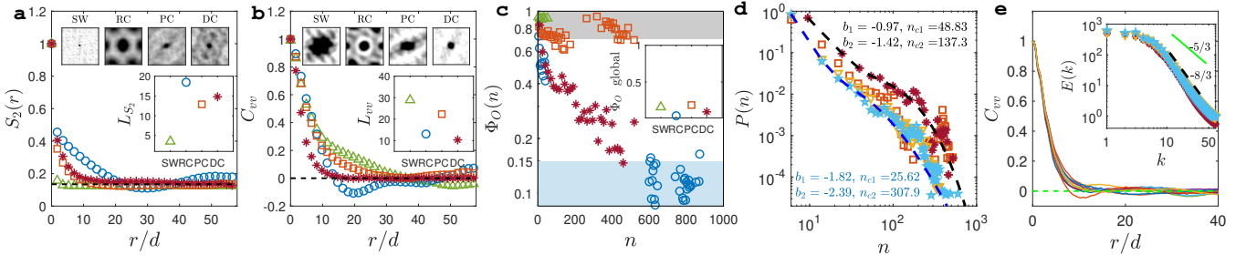
FIG. 4. (a) Angular-averaged normalized two-point correlation vs. normalized radial distance r ; top inset: in 2D, showing the spatial periodicity of rotating cluster; bottom inset: characteristic length of S_2 . Angular-averaged velocity auto-correlation vs. normalized radial distance; top inset: in 2D, showing the periodicity of velocity correlation of rotating and polar clusters in space. Some degree of anisotropy in the velocity auto-correlation of polar cluster is due to insufficient number of clusters in the field of view; bottom inset: characteristic length of C_{vv} . (c) Polar order parameter vs. n , the number of particles in a cluster; inset: global order parameter; shaded areas indicate polar ordering higher than 75% and lower than 15%. (d) Probability distribution of clusters with n number of particles. (e) VACF of a disordered cluster with \tau_R = 100 ms evaluated at different run steps. Inset: Angular-averaged energy spectrum of disordered clusters. Symbols denote different phases: \square : polar cluster (PC) ( \tau_T/\tau_{mw} = 3, \tau_R = 8 ms), * : disordered cluster (DC) ( \tau_T/\tau_{mw} = 10, \tau_R = 40 ms), \nabla : disordered cluster ( \tau_T/\tau_{mw} = 10, \tau_R = 100 ms), * : disordered cluster ( \tau_T/\tau_{mw} = 10, \tau_R = 150 ms), \Delta : swarm (SW) ( \tau_T/\tau_{mw} = 1, \tau_R = 4 ms)
