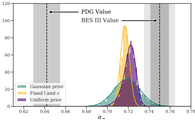
FIG. 1. Posterior densities for \alpha_- , given different priors for the beam polarization calibration constants P_C^\gamma and P_L^\gamma . The histograms show the result of the MCMC sampling of the marginalized posterior densities while the solid lines represent a direct scan of the posteriors. For clarity, the results corresponding to the double width uniform priors for P_C^\gamma and P_L^\gamma are omitted. Dark grey vertical bands represent statistical uncertainty; the additional light grey bands on the BESIII result represent systematic uncertainty.
