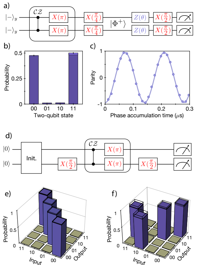
FIG. 3. Bell state preparation and CNOT gate. a) Quantum circuit used to prepare and probe the |\Phi^+\rangle state. b) Measured populations of the Bell states. Raw measurements associating |0\rangle with atom presence and |1\rangle with atom absence yields 97.6(2)% in the target states. Separate measurements of leakage out of the qubit subspace indicate a small contribution (light shaded region) to these probabilities; subtracting this contribution, the measured population is \geq 95.8(3)\% . c) The parity oscillation with respect to accumulated phase \theta has a measured amplitude of 94.2(4)%. The resulting lower bound on Bell state fidelity is \mathcal{F} \geq 95.0(2)\% (raw measurements yield \mathcal{F}^{\text{raw}} = 95.9(2)\% ). Correction for SPAM errors results in \mathcal{F}^c \geq 97.4(3)\% . d) The CNOT gate is constructed from our native CZ gate with the addition of local hyperfine qubit rotations. e) The four computational basis states are prepared with average fidelity 96.8(2)%. f) We apply the CNOT sequence to the four computational basis states and measure the truth table fidelity to be \mathcal{F}_{\text{CNOT}} \geq 94.1(2)\% . Corrected for SPAM errors, the fidelity is \mathcal{F}_{\text{CNOT}}^c \geq 96.5(3)\% . Wireframes on purple bars show ideal outcomes; solid bars show the raw measurement; the light-shaded top portions of the bars bound the contribution from qubit leakage. Only the darker lower region is counted towards fidelities.
