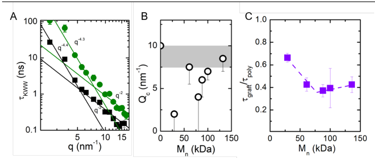
Figure 2: (A) Comparison of the q -dispersion curves for a composite with M_n \approx 88 \text{ kDa} (black \blacksquare ) and a bulk polymer with M_n = 96 \text{ kDa} (green \bullet ). (B) Crossover q 's ( \circ ) for the two asymptotic behaviors observed for the different grafted samples. The grey band corresponds to the crossover wavevectors for the bulk polymer. The M_n \approx 29 \text{ kDa} (HFBS) and M_n \approx 80 \text{ kDa} (SPHERES) have no evidence for a crossover within instrument parameters – the error bars extending to zero on the y-axis point to this fact. The point at zero molecular weight is the pure PMA (with no NPs). (C) Relaxation times of the composites normalized to the bulk polymer after summing across all wavevectors. The dashed line is a guide to the eye. Data was measured on HFBS.
