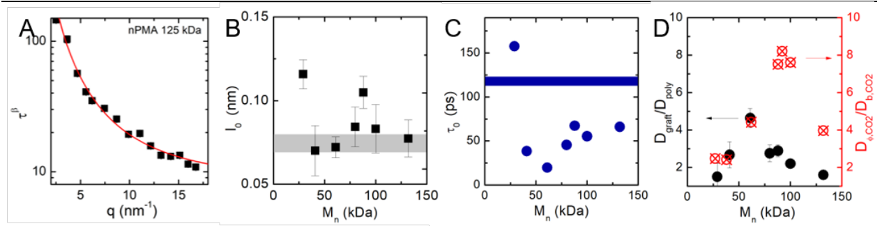
Figure 3: (A) \tau^\beta vs q with fits to the jump diffusion model (solid line). (B) Jump length, l_0 , extracted from the model for all composites tested. The grey band corresponds to the jump length for the reference polymer melt (no NPs). (C) Relaxation time \tau_0 for the diffusive jumps. The bands represent the corresponding fit values for the reference polymer melt. (D) Normalized segmental diffusivity for the composites (Black \bullet ). Normalized diffusivities of CO 2 in the GNPs are plotted (Red symbols) as a function of M_n . Similar non-monotonic behavior is observed for the two, although quantitative differences persist.
