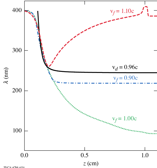
Figure 5. A plot of minimum vacuum wavelength over propagation distance, displayed for four separate ionization front velocities. Drawn in a green dotted line is a reproduction of the simulated case in (a), with a flying focus focal velocity of v_f = c ; in a red dashed line is a superluminal case in which v_f = 1.1c ; in a blue dash-dotted line is a subluminal case in which v_f = 0.9c ; in a black solid line is a case in which no flying focus is formed, and instead, the ionization front travels at the group velocity of the drive pulse v_d = 0.96c .
