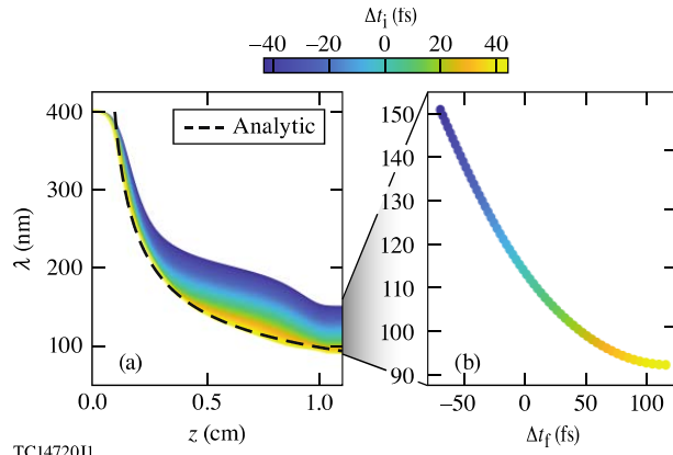
Figure 4. (a) A plot of vacuum wavelength, \lambda , over propagation distance, z , for a pulse modeled by a series of photons evenly distributed over an input duration of 87 fs, each with a color corresponding to the initial temporal location within the pulse, \Delta t_i (colorbar). For comparison, the analytic case is plotted for the highest-frequency photon (dashed black line). (b) The distribution of wavelength over the final duration of the witness pulse, \Delta t_f , for the simulated case shown in (a).
