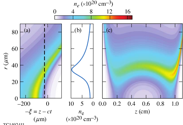
Figure 2. Profiles of the plasma guiding structure created when the flying focus drive pulse ionized the shaped gas target. (a) The transverse profile as a function of moving frame coordinate -\xi = z - ct at z = 0.7 \text{ cm} . (b) a line out corresponding to the dashed line in (a). (c) the guiding profile experienced by a typical photon within the witness pulse along the length of the accelerator (i.e. at each z , the transverse profile was extracted at the \xi -location of the photon).
