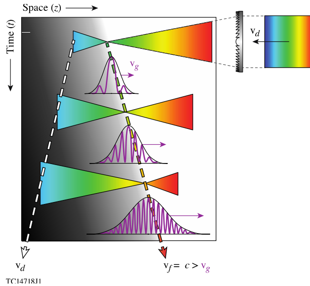
Figure 1. A schematic demonstrating photon acceleration in the ionization front of a flying focus. A negatively chirped drive pulse propagating at its group velocity, v_d < 0 , forms a focus that counter-propagates at the velocity, v_f = c , triggering an ionization front traveling at c . The resulting electron density is indicated by shading. A witness pulse (drawn in purple) copropagates with the ionization front at velocity v_g and continually upshifts in frequency.
