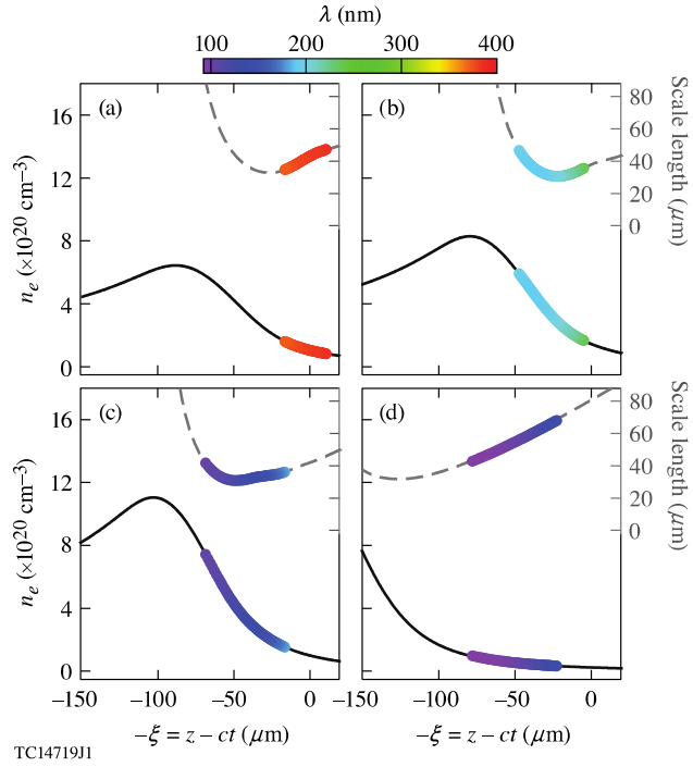
Figure 3. A series of snapshots of an 87 fs witness pulse with an initial wavelength \lambda = 400 nm copropagating with a temporal gradient in the electron density. The snapshots are taken at propagation distances of (a) 0.10, (b) 0.30, (c) 0.8, and (d) 1.05 cm and plotted in the moving frame, \xi . The pulse is modeled by photons initially spaced evenly in time over 87 fs. Each photon is represented by a circle colored to correspond to its vacuum wavelength (colorbar). The electron density and scale length, L = n_e / \partial_\xi n_e , are shown as solid black and dashed gray lines respectively.
