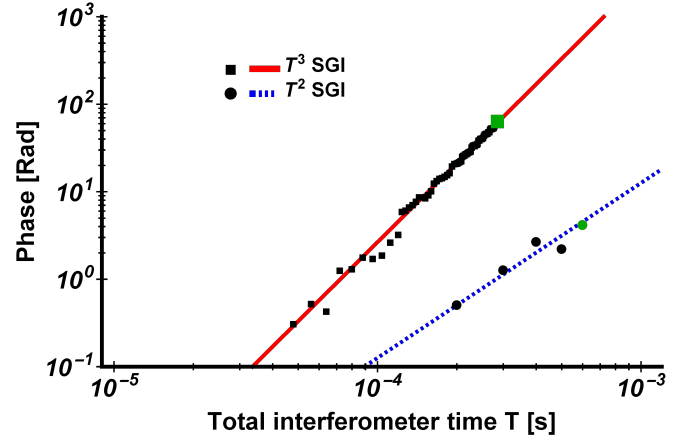
FIG. 3. Comparison between the scalings of the interferometer phases \delta\Phi^{(T^3)} (solid red curve) and \delta\Phi^{(T^2)} (dashed blue curve) given by Eqs. (10) and (11), respectively. The squares are data from Fig. 2, while the dots are from our T^2 -SGI realization [11]. The green square represents the largest accumulated phase of the T^3 -SGI in its current configuration with T_{\max} = 285 \mu\text{s} at the point of \approx 30\% contrast. As a reference, the green dot indicates the largest accumulated phase observed with a T^2 -SGI also at \approx 30\% contrast. The latter is significantly smaller although the magnetic field gradients and the maximal time T_{\max} = 924 \mu\text{s} are larger than those of the T^3 -SGI by a factor of 2.3 and 3.2, respectively [36].
