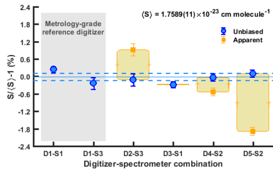
Fig. 3. Unbiased ( S , blue circles) and apparent ( S_A , orange squares) values of the R 16e \text{CO}_2 line intensity at T = 296 K (30012 – 00001 band). Error bars show \pm 1\sigma standard uncertainties. The gray shaded region comprising D1-S1 and D1-S3 (far left) highlights values of S measured by the metrology-grade reference digitizer. For values of S with corresponding values of S_A , light orange boxes indicate the magnitude of each digitizer correction. The light blue dashed lines bound the standard deviation of the weighted mean value of \langle S \rangle (solid blue line).
