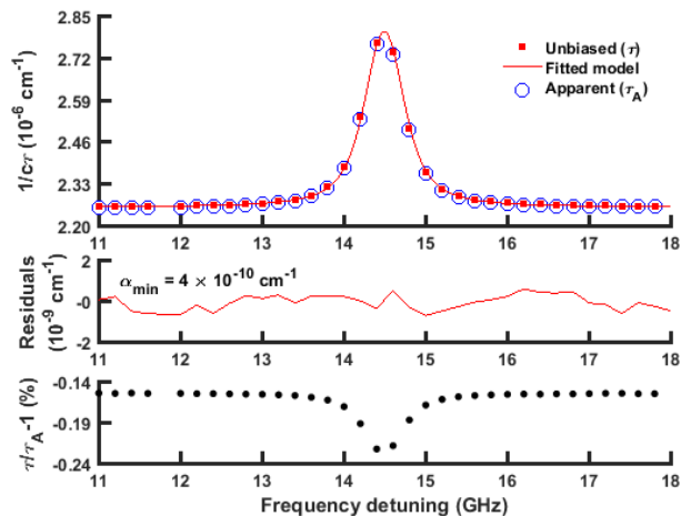
Fig. 2. A portion of representative unbiased (red squares) and apparent (blue circles) spectra of the R 16e \text{CO}_2 transition with \tilde{\nu}_0 = 6359.967 \text{ cm}^{-1} are shown in the top panel. Fitted spectra spanned a frequency detuning range of 0 GHz to 28 GHz, the sample pressure was 8.88 kPa, and the sample \text{CO}_2 mole fraction was \chi_{\text{CO}_2} = (387.98 \pm 0.05) \mu\text{mol/mol} . The apparent spectrum was recorded by the digitizer-spectrometer combination D4-S2, and \tau_A were corrected to yield \tau using the coefficients in the Supplemental Material [43]. A fitted model of the unbiased absorption coefficient ( \alpha = 1/c\tau ) is also shown as a red line and fitted residuals are plotted as another red line in the middle panel. In the bottom panel, the relative difference \tau/\tau_A - 1 (equal to \alpha_A/\alpha - 1 , where \alpha_A is the apparent absorption coefficient) is plotted as black dots.
