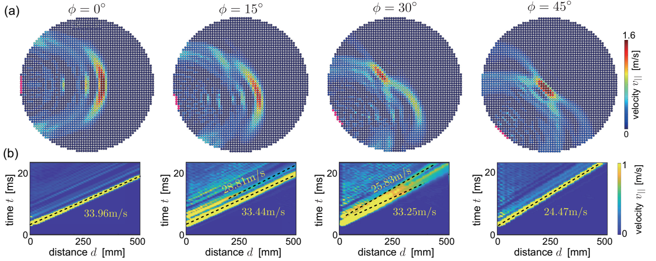
FIG. 2. Numerical results for a circular model with 60 squares along its diameter. (a) Contour plots of v_{||} at t = 12 ms for all four impact angles. (b) Spatial-temporal map of v_{||} for all considered impact angles. The magenta squares in (a) are those to which the displacement is applied. The full time evolution is available in Movie S2.
