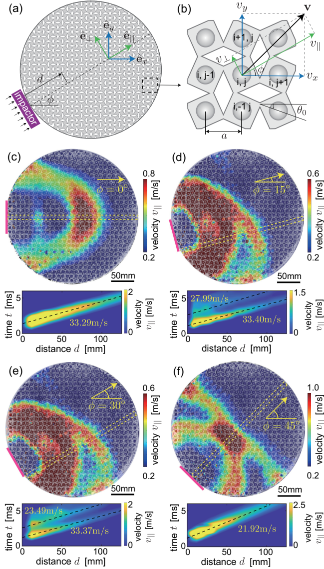
FIG. 1. (a) Schematic of the system. (b) Definition of velocity of squares. (c)-(f) Contour plots of parallel velocity v_{\parallel} and t-d contour plots of velocity along indicated direction for impact angles of \phi = 0^\circ , 15^\circ , 30^\circ and 45^\circ . The magenta squares are those to which the displacement is applied. The full time evolution is available in Movie S1.
