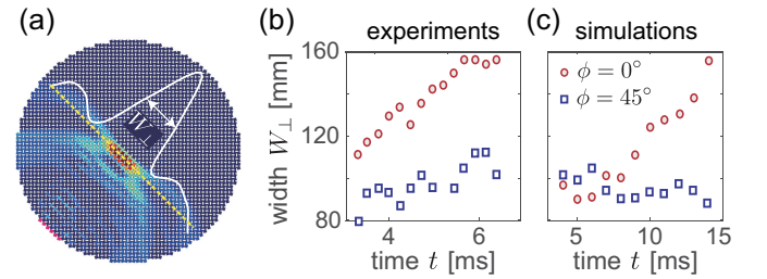
FIG. 4. (a) Schematic highlighting the full width at half maximum, W_{\perp} . (b)-(c) Time evolution of W_{\perp} as extracted from (b) experiments and (c) simulations for \phi = 0^\circ (red markers) and \phi = 45^\circ (blue markers).
