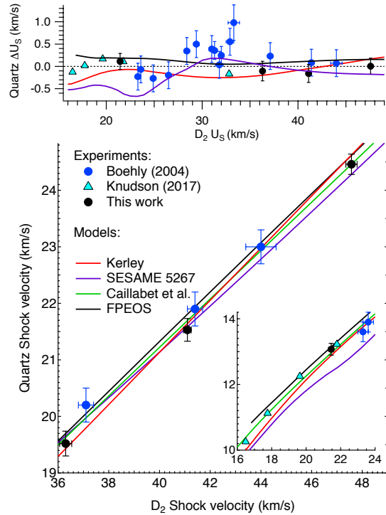
FIG. 3. (Color online) Reflected-shock observables, U_S^Q vs U_S^D , from this study are shown as black filled circles. Previous laser-driven data from Ref. [43] are shown in blue filled circles and recent flyer plate measurements from Ref. [20] are shown in cyan triangles. All experimental data are plotted with error uncertainties. The colored solid lines correspond to the predictions of four EOS models. Note that the main plot covers the velocity range 36 < U_S^D < 50 km/s while the inset covers the 16 < U_S^D < 24 km/s. Top: Velocity residuals of the different data sets and EOS models with respect to the Caillabet et al. model.
