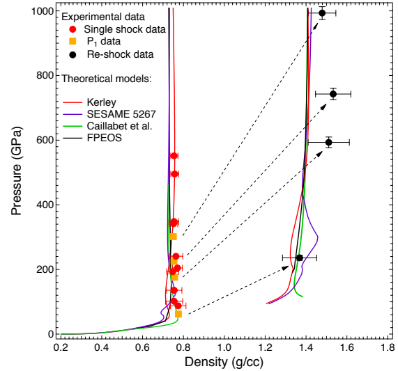
FIG. 4. (Color online) Single-shock and reflected-shock compressed densities of cryogenic liquid deuterium. The orange squares correspond to ( P_1, \rho_1 ) states, the shock state in D_2 prior to reflection from the quartz anvil (as the shock wave was not steady [32]). The red circles correspond to the single-shock data shown in Fig.2 and the black circles correspond to the D_2 reshock states. The dashed arrows are guides to the eye and they link the single and reflected-shock states. The solid color lines correspond to four EOS models (as in Fig. 2).
