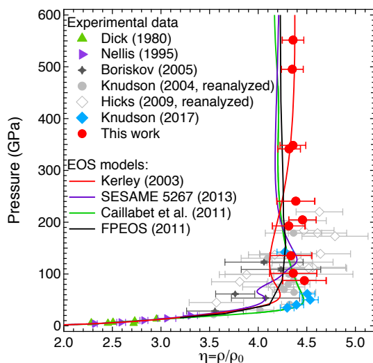
FIG. 2. Pressure versus compression for single-shock measurements of the principal Hugoniot of cryogenic liquid deuterium. Impedance-match results from explosive-driven flyer-plate impact [40] (green triangles), gas gun [41] (purple triangles), explosive-driven hemispherical shell-impact [42] (dark grey stars), magnetically-driven flyer-plate [13] (gray circles), laser-driven [14] (open gray diamonds), magnetically-driven flyer-plate [20] (blue diamonds) and laser-driven measurements (this work, red circles) are shown. The data are compared to several EOS models: Kerley [37] (solid red curve), Sesame 5267 [38] (solid purple curve), Caillabet et al. [35] (solid green curve) and FPEOS [39] (solid black curve).
