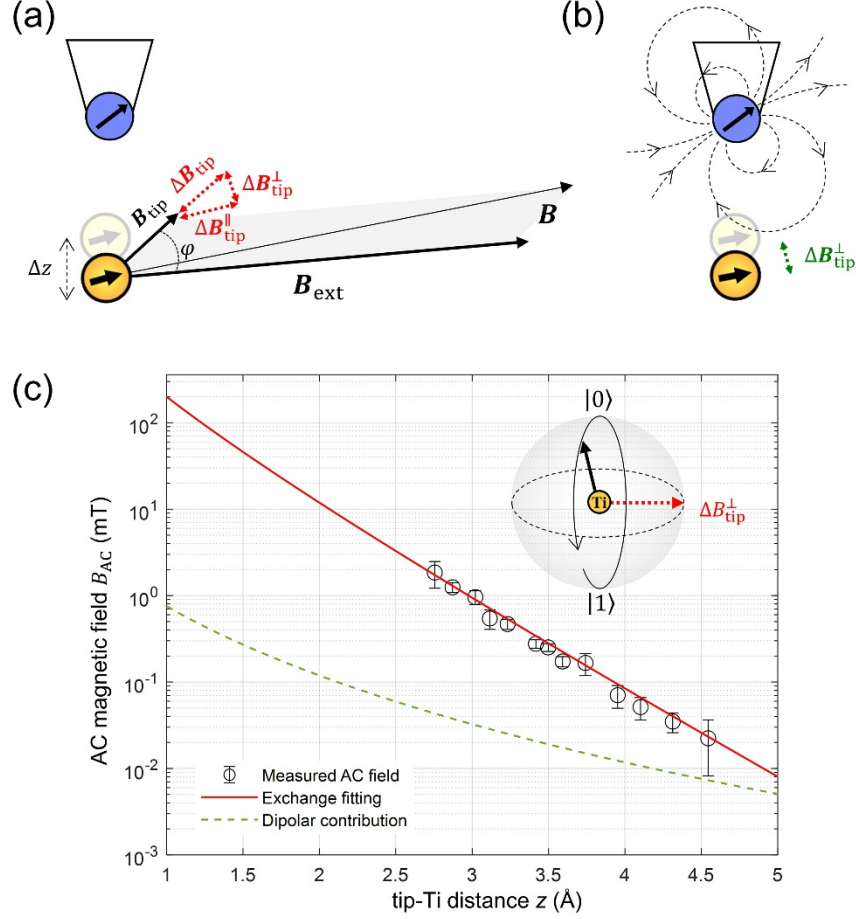
FIG. 4. Driving ESR by varying tip-Ti magnetic interactions. (a) and (b), Schematic of two possible ESR driving mechanisms: modulation of the (a) exchange and (b) magnetic dipolar interactions. (c) Extracted AC magnetic field as a function of tip-Ti distance z at V_{\text{RF}} = 10 mV. Red solid curve is the fit considering exchange interactions (with \varphi \approx 60^\circ ). The green dashed curve is the calculated AC magnetic field from dipolar interaction. Inset shows the rotation of the Ti spin (solid black arrow) around the AC tip field (dashed red arrow) between |0\rangle and |1\rangle states in a Bloch sphere in the rotating frame.
