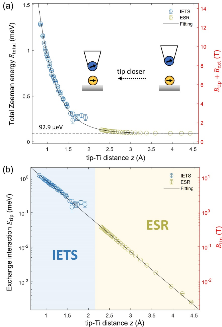
FIG. 3. Exchange interaction as a function of tip-to-atom distance. (a) E_{\text{total}} of a single Ti atom under a magnetic tip as a function of the tip-Ti distance. Symbols represent the Zeeman energy determined from IETS (blue circles) and ESR (light-green circles). The solid line is an exponential fit. The asymptotic value is 92.9 \mu\text{eV} indicated by the dashed line. (b) E_{\text{tip}} and B_{\text{tip}} as a function of the tip-Ti distance (log scale on the y axes). The data are extracted from (a) by subtracting the asymptotic value. The solid line is an exponential fit. The error bars are determined by the fitting uncertainties of the IETS step positions and the ESR frequencies.
