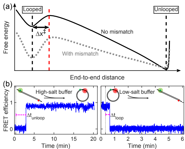
FIG. 1. (a) Schematic illustration of a free energy landscape for DNA loop capture and release. The two minimum free energy states correspond to the looped and unlooped states (vertical black lines). The transition state (vertical red line) is separated from the looped state by a small distance \Delta x^\ddagger , which is equal to the capture radius. The base pair mismatch is expected to increase until the solid curve toward shorter end-to-end distances, which results in the dotted curve. (b) Typical FRET trajectories of a DNA molecule undergoing loop capture (left) and loop release (right). The DNA molecule labeled with Cy3 (green) and Cy5 (red) is in the low FRET state when unlooped, and in the high FRET state when looped. A sudden increase or decrease in NaCl concentration at the 20-second time point (marked by a vertical dotted line) triggers the transition.
