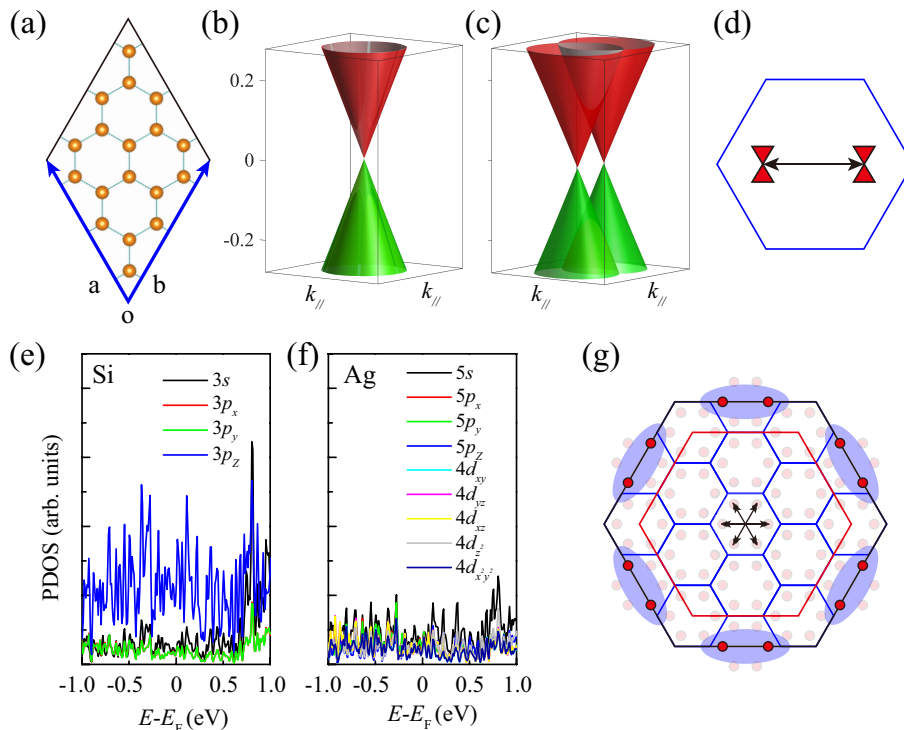
FIG. 3. (Color online) (a) Schematic illustration of the periodic potential in our tight-binding model. (b) and (c) Calculated band structures using the tight-binding model before (b) and after (c) applying the periodic potential. (d) Schematic drawing of the splitting direction of the Dirac cone. (e) and (f) Calculated partial density of states of Si and Ag atoms, respectively, using DFT. (g) Schematic drawing of the Dirac cone pairs in the BZs of silicene and Ag(111). The red dots represent the positions of the Dirac cones. The blue shaded ellipses highlight the Dirac cones that have been experimentally observed. The black double arrows indicate the splitting of the Dirac cones.
