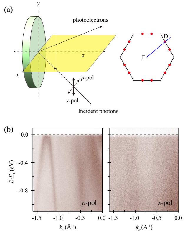
FIG. 2. (Color online) (a) Left panel: schematic illustration of the experimental geometries of the ARPES measurements. The incident light lies in the detection plane (colored yellow). The s and p polarization is defined as perpendicular and parallel to the detection plane, respectively. Right panel: schematic drawing of the BZ of Ag(111) and the positions of the Dirac cones. The blue line indicates the momentum cut that includes the \Gamma point and Dirac point. (b) ARPES intensity plots along the blue line with p and s polarized light, respectively. The incident photon energy is 50 eV.
