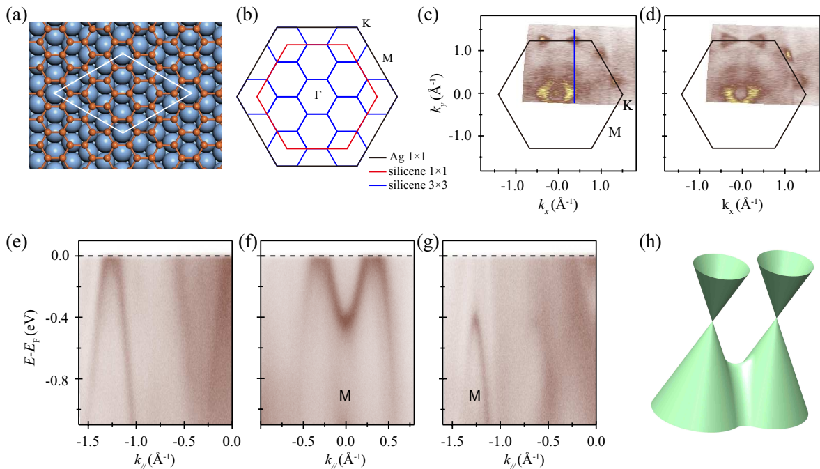
FIG. 1. (a) (Color online) Atomic structure of 3\times 3 silicene on Ag(111). Orange and blue balls represent Si and Ag atoms, respectively. The white rhombus indicates a unit cell of the 3\times 3 superstructure. (b) BZs of silicene (red lines), Ag(111) (black lines), and the superstructure (blue lines). (c) Photoemission intensity at the Fermi level as measured with 50 eV p -polarized photons. The blue line indicates the momentum cut along which the ARPES intensity plots in (e) were taken. (d) The same plot as in (c) but at a binding energy of 0.2 eV. (e-g) ARPES intensity plot along the blue line in (c), along the \bar{K} - \bar{M} - \bar{K} direction, and along the \bar{\Gamma} - \bar{M} direction, respectively. (h) Schematic drawing of a pair of Dirac cones.
