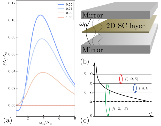
FIG. 1. (Color Online) (a) Relative enhancement of the gap function as a function of cavity frequency \omega_0 for a particular value of the overall scaling constant \pi\alpha X D T_{\text{in}}/c^2 (we take X = 133 and \pi\alpha D T_{\text{in}} T_c^2/c^2 = 9.17 \times 10^{-5} with T_c set to unity). Curves are colored and labeled according to the ratio T_{\text{cav}}/T_{\text{qp}} , comparing the photon and quasiparticle temperatures. The enhancement is seen set in after the cavity frequency surpasses the pair-breaking energy 2\Delta_0 . (b) Schematic picture of the system used for calculation. The lowest cavity resonator mode with cutoff frequency \omega_0 is shown. (c) Depiction of the various processes which contribute to the quasiparticle collision integral, plotted against the equilibrium n(E) . The blue arrows depict the down-scattering terms captured by f(\Omega, E) , the red arrows depict the up-scattering terms captured by f(-\Omega, E) and the green arrows represent the pair-processes captured by f(-\Omega, -E) .
