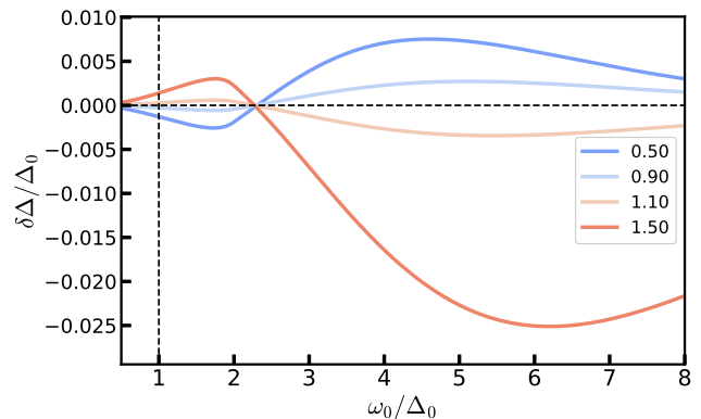
FIG. 3. (Color Online) Gap enhancement \delta\Delta_0 for a single-mode cavity, for both cold and hot photons. The y-axis is determined by the overall scale 4\pi\alpha D\tau_{\text{in}}T_c^2/((\pi\sqrt{3})^3c^2)X ; with the same values chosen for X and \tau_{\text{in}}, \tau_{\text{el}}, v_F/c as in Fig. 1. Curves are colored and labeled according to the ratio T_{\text{cav}}/T_{\text{qp}} , comparing the photon and quasiparticle temperatures. Here the cavity width is held fixed at 1/2\tau_{\text{cav}} = 10\omega_0 .
