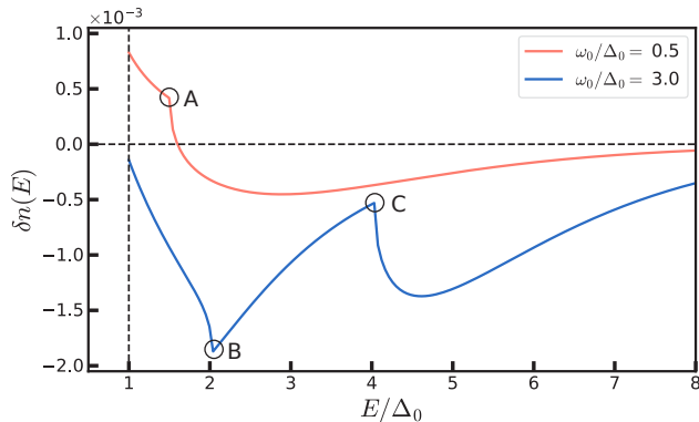
FIG. 2. (Color Online) Change in quasiparticle distribution function due to cavity photons. The two curves are at the same temperature ( T_{\text{cav}}/T_{\text{qp}} = 0.5 ) but different cavity frequencies \omega_0/\Delta_0 . For low cavity frequency (orange), the gap \Delta is diminished due to an accumulation of cooler quasiparticles near the gap-edge, due to a down-scattering of particles. For higher cavity frequency (blue), the recombination processes are more dominant and lead to a net reduction in quasiparticles, enhancing the gap \Delta . The kink-features labeled A and C reflect the onset of the term f(\Omega, E) in Eqn. (14), which is only non-zero for E > \omega_0 + \Delta_0 . At higher cavity frequencies ( \omega_0 > 2\Delta_0 ) an additional kink-feature (located at B ) emerges at E = \omega_0 - \Delta_0 . For E < \omega_0 - \Delta_0 , the term f(-\Omega, E) (which represents the pair-processes) contributes over the entire integration region of \Omega > \omega_0 , while for E > \omega_0 - \Delta_0 the integral only captures some of the frequencies where this term contributes.
