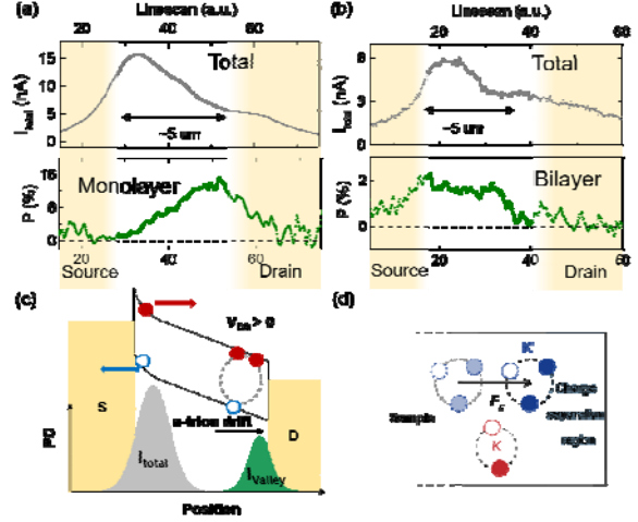
FIG. 4. (a) Spatial distribution of photocurrent across the source and drain contacts for monolayer sample at 16\text{T} . Gray line in upper panel indicates the total photocurrent distribution. The non-zero tails at the end of contacts are due to the large laser spot ( \sim 2\mu\text{m} ) and residual scattered light. The corresponding polarization P which mainly comes from the valley contribution, is plotted in the lower panel in green. (b) Same measurements and notations as (a) measured in bilayer \text{MoS}_2 . Spatial distribution for P now mainly reflects the spin polarization contribution. (c) Schematics of the material's bands across the device at the given experimental condition ( n -doping, V_{DS} > 0 ). The bands near the source has a higher band bending. Correspondingly, we have a higher I_{\text{total}} near the source contact, as indicated by the grey area. The applied electric field would drift the valley polarized n -trions towards drain contacts, creating a higher valley photocurrent denoted by green. (d) Schematics for transport scenario comparing the trions and neutral excitons of different valleys.
