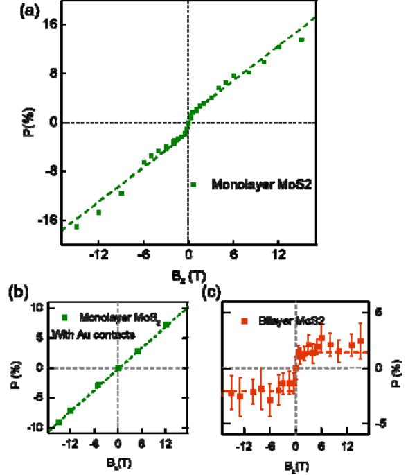
FIG. 2. (a) The polarization dependence P of photocurrent plotted as a function of magnetic field for monolayer MoS 2 ( n -type) with ferromagnetic contact. Two distinct regimes of response can be seen. (b) The corresponding magnetic-field dependence of P for monolayer MoS 2 with Au contacts and (c) bilayer MoS 2 (2H, n -type) with ferromagnetic contacts.
