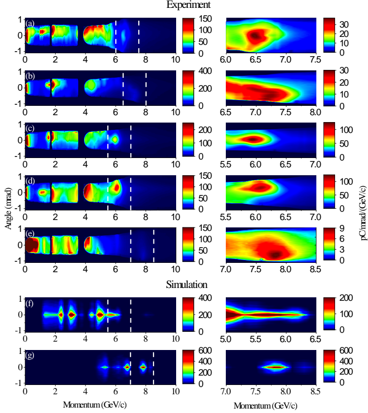
FIG. 4. (a)–(e): Electron beams measured by the magnetic spectrometer for n_0 = 3.4 \times 10^{17} \text{ cm}^{-3} , r_m = 69 \text{ } \mu\text{m} and laser power 850 TW. The driver laser pulse arrival was timed with the peak of the heater pulse. The heater pulse arrived 300 ns after the peak of the discharge current, except for (e), where the delay was 420 ns, and the heater-induced density reduction was measured to be larger, with n_0 = 2.7 \times 10^{17} \text{ cm}^{-3} and r_m = 61 \text{ } \mu\text{m} . The white dashed lines show the regions that are plotted in the right hand column, which shows the detailed spectrum of the highest energy peaks. The electron beam spectrum simulated by INF&RNO using the MARPLE-retrieved density profile (with n_0 = 3.4 \times 10^{17} \text{ cm}^{-3} ) is shown in (f). In (g) a simulation is shown for the parameters of (e) using a transversely parabolic and longitudinally uniform density profile.
