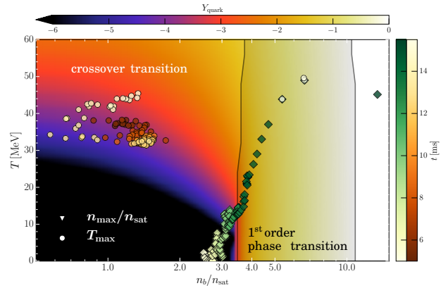
FIG. 3. Evolution of the maximum normalized baryon number density (diamonds) and temperature (circles) after the merger for the low-mass binary with the \text{CMF}_Q EOS. Different times of the evolution are represented with a color code, together with the quark fraction Y_{\text{quark}} . The grey shaded area shows the first-order PT region.
