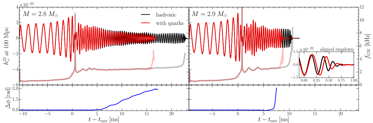
FIG. 4. Properties of the GW emission for the low- (left panels) and high-mass binaries (right panels). The top panels report the strain h_+^{22} for the two EOSs, together with the instantaneous GW frequency f_{\text{GW}} (semitransparent lines); the bottom panels show the phase difference \Delta\phi between the two signals. The inset in the top-right panel highlights the differences in the ringdown.
