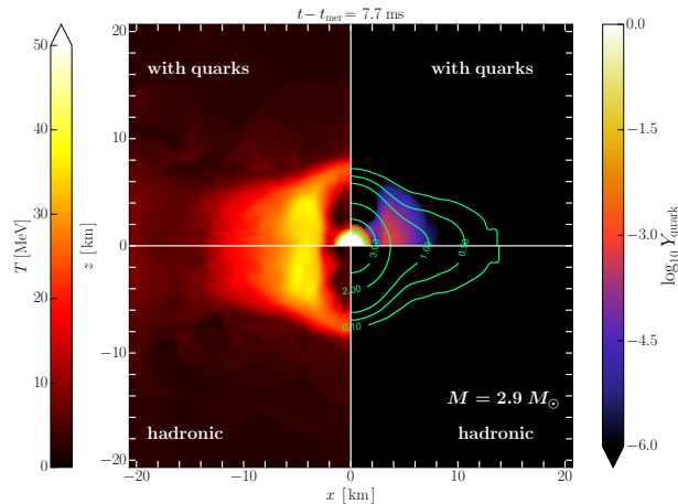
FIG. 2. Same as Fig. 1 but on the meridional plane; the top/bottom panels show simulations with the \text{CMF}_Q/\text{CMF}_H EOSs, respectively. The snapshot refers to the high-mass binary at a time shortly before the collapse to a black hole.
