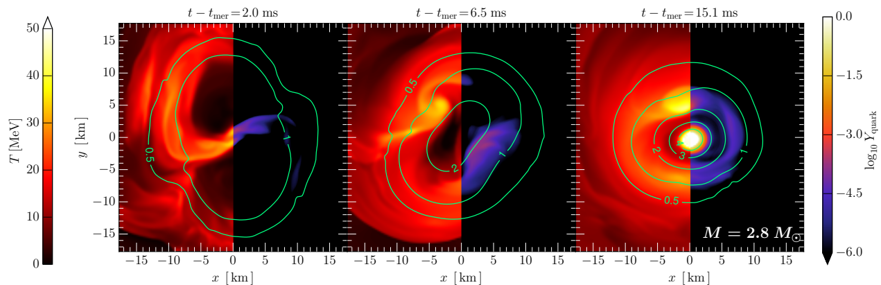
FIG. 1. Snapshots on the equatorial plane at three representative times of the evolution of the low-mass binary. For each snapshot, the left part of the panel reports the temperature T , while the right part reports the quark fraction Y_{\text{quark}} . The green lines show contours of constant number baryon density in units of the nuclear saturation density n_{\text{sat}} . Note that a PT takes place only shortly before the HMNS collapses to a black hole (cf. right panel).
