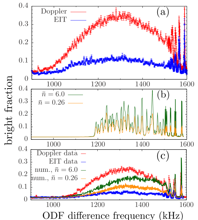
FIG. 4. Scan over all the axial drumhead modes. a) Data taken after Doppler cooling (red) and after Doppler and EIT cooling for 200 \mu\text{s} (blue) for a crystal with 158 \pm 10 ions. b) Theoretical calculation of the bright fraction for a crystal with N = 79 ions after Doppler cooling (green) and subsequent EIT cooling (orange). c) Comparison of the measured (red, blue) and the theoretically calculated (green, orange) bright fraction for a crystal with N = 79 \pm 5 ions and t_{\text{EIT}} = 300 \mu\text{s} . The calculation took into account mode frequency instabilities leading to the loss of visibility of individual modes, and a 5% uncertainty in the ODF amplitude F .
