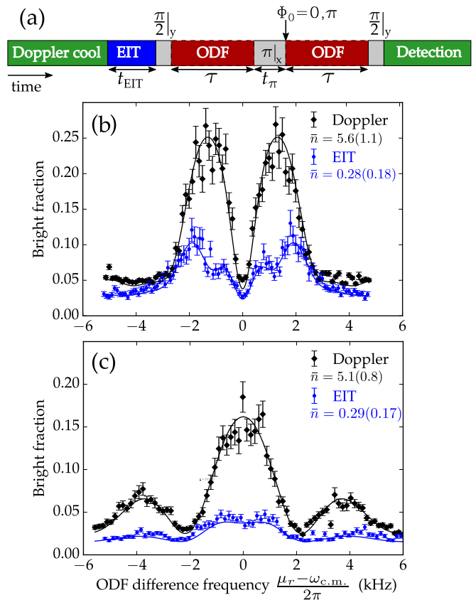
FIG. 2. a) Experimental pulse sequence. \pi and \pi/2 pulses are implemented with resonant microwaves, \Phi_0 is the phase shift between the two ODF pulses. b) Temperature measurement of the c.m. mode at frequency \omega_{\text{c.m.}} = 2\pi \times 1.59 MHz for a crystal with 158 \pm 10 ions. The black diamonds are the measured fraction of ions in the |\uparrow\rangle state after Doppler cooling only, and the blue dots after Doppler cooling followed by 200 \mu\text{s} of EIT cooling. The solid lines are least squares fits of Eq. (1) to the data, the fitted mean c.m. mode occupations are given in the legend. The ODF interaction time was 2\tau = 500 \mu\text{s} . The increased background after only Doppler cooling is due to a larger measured \Gamma resulting from weak Lamb-Dicke confinement. c) Same as b) but with \Phi_0 = \pi and 2\tau = 300 \mu\text{s} .
