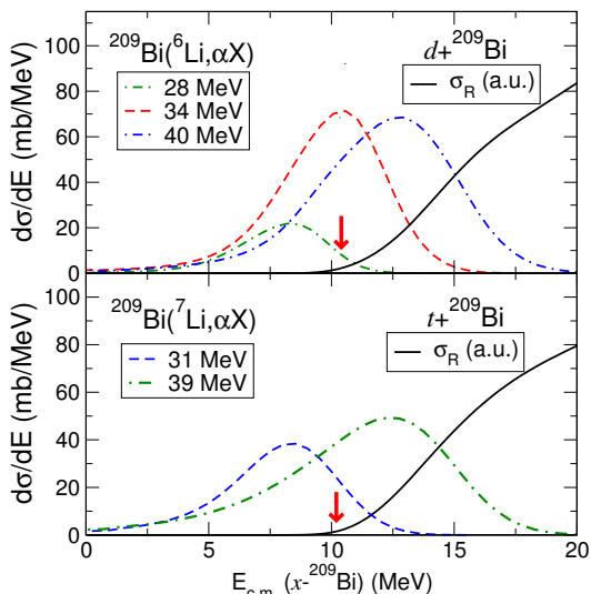
FIG. 4. Illustration of the Trojan Horse mechanism for the ^{209}\text{Bi}(^6\text{Li}, \alpha X) (upper panel) and ^{209}\text{Bi}(^7\text{Li}, \alpha X) (lower panel) reactions. The broken lines are the three-body cross sections ( ^{6,7}\text{Li}, \alpha X ) at the incident energies indicated by the labels. The black solid lines are the two-body reaction cross sections (in arbitrary units). The nominal position of the barrier for the d+^{209}\text{Bi} and t+^{209}\text{Bi} reactions is indicated by the arrows.
