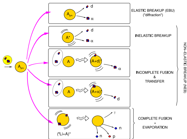
FIG. 1. Illustration of transfer/breakup modes for a {}^6\text{Li} + A reaction. See text for details.
