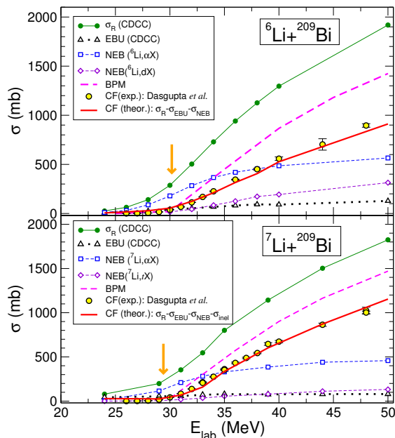
FIG. 2. Complete fusion cross section for the ^{6,7}\text{Li}+^{209}\text{Bi} reactions as a function of the incident energy. Experimental data are from Ref. [4]. The arrow indicates the nominal position of the Coulomb barrier.
