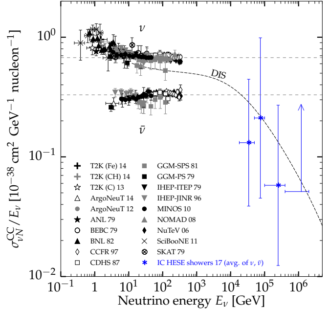
FIG. 1. Charged-current inclusive neutrino-nucleon cross section measurements [8–25]. The new results from this work, based on 6 years of IceCube HESE showers [26–29], are an average between cross sections for \nu and \bar{\nu} , assuming equal astrophysical fluxes of each. In the highest-energy bin, we only set a lower limit ( 1\sigma shown). The thick dashed curve is a standard prediction of deep inelastic scattering (DIS), averaged between \nu and \bar{\nu} . Horizontal thin dashed lines are global averages from Ref. [30], which do not include the new results.
