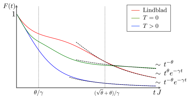
FIG. 1. (Color online) Comparison between the fidelity F(t) for a quantum Ising chain with a spin-dephasing impurity (red line) and for the same Ising chain with a local defect on the transverse field, at zero temperature [29] (green line) and at finite temperature [30] (blue line). The asymptotic behavior of the three curves is highlighted on the right. The local lindbladian channel results in a slower decay of the fidelity compared to the other two cases. Close to t \lesssim (\sqrt{\theta} + \theta)/\gamma the fidelity in the dissipative Ising model transits from a concave universal behaviour to the usual convex character typical of isolated systems.
