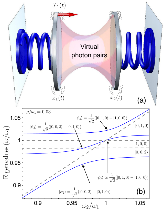
Figure 1. (a) Schematic of an optomechanical system constituted by two vibrating mirrors. If one of the two vibrating mirrors is excited by an external drive \mathcal{F}_1(t) , its excitation can be transferred coherently and reversibly to the other mirror. The interaction is mediated by the exchange of virtual photon pairs. (b) Relevant energy levels of the system Hamiltonian \hat{H}_s as a function of the ratio between the mechanical frequency of mirror 2 and that of mirror 1. An optomechanical coupling g/\omega_1 = 0.03 has been used; the cavity-mode resonance frequency is \omega_c = 0.495\omega_1 . The lowest energy anti-crossing corresponds to the resonance condition for the DCE [26]. The higher energy one is the signature of the mirror-mirror interaction mediated by the virtual DCE photons.
