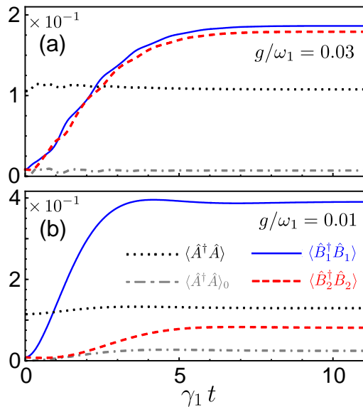
Figure 2. System dynamics for \omega_c \simeq 1.5\omega_1 under continuous-wave drive of mirror 1. The blue solid and red dashed curves describe the mean phonon numbers \langle \hat{B}_1^\dagger \hat{B}_1 \rangle and \langle \hat{B}_2^\dagger \hat{B}_2 \rangle , respectively, while the black dotted curve describes the mean intracavity photon number \langle \hat{A}^\dagger \hat{A} \rangle and the grey dash-dotted curve shows the same photon number \langle \hat{A}^\dagger \hat{A} \rangle_0 , calculated assuming zero temperature.
