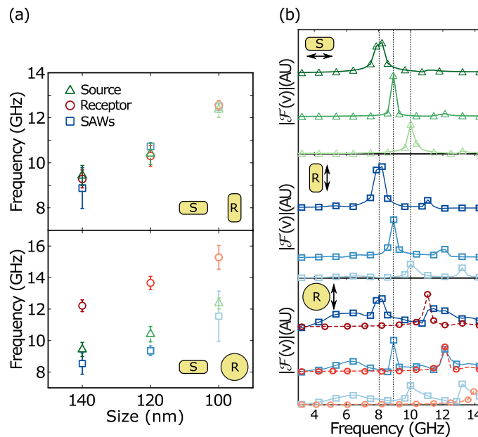
FIG. 4. (a) Averaged experimental frequencies of rod sources (60 nm width, 30 nm height - green triangles), and rod (60 nm width, 30 nm height, top) or disk (30 nm height, bottom) receptors (R - red circles) of indicated main-axis size (diameter for disks). Stronger colors correspond to larger sizes. Blue squares indicate the measured SAWs-induced probe modulation frequencies at the receptor when the pump beam is set at the source. (b) FEM time-domain Fourier components of the size variation along the axes parallel to the probe beam polarization (black arrows) for the rod source (top), and rod (middle) and disk (bottom) receptors. Vertical dashed lines correspond to extensional modes of the sources. Disk radial modes are shown in red dashed lines/circles (bottom).
