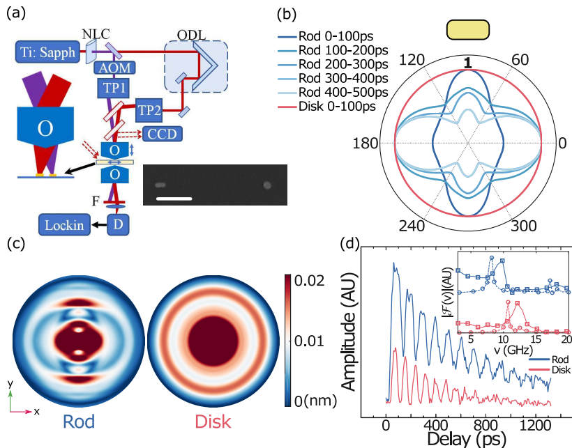
FIG. 1. (a) Schematic representation of pump-probe experiment. NLC: non-linear crystal, ODL: optical delay line, AOM: acousto-optic modulator, O: microscope objective, D: photodetector, TP: telescope and position adjustment. (inset) SEM image of a rod source and a disk receptor 1.5\mu\text{m} distant. Scale bar corresponds to 500\text{ nm} . (b) FEM average displacement at the edge of the simulation region of a 140 \times 60 \times 35\text{ nm} rod (blue, 0 - 500\text{ ps} ) and a 140 \times 35\text{ nm} disk (red, 0 - 100\text{ ps} ). Rod orientation is shown on top. (c) Substrate displacement at t = 50\text{ ps} . Antennas omitted for clarity. (d) Modulated probe transmission of single antennas. (inset) Fourier transform of probe signals (solid-square lines) and FEM size variations along x-axis (dashed-circle lines).
