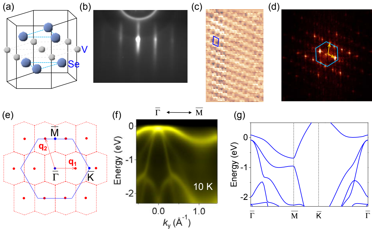
FIG 1. Film structure, electronic band structure, and STM images of single-layer \text{VSe}_2 . (a) Atomic structure of single-layer 1T \text{VSe}_2 . (b) A RHEED pattern taken at room temperature after single-layer \text{VSe}_2 film growth. (c) A STM topographic image taken from single-layer \text{VSe}_2 at 77 K revealing (\sqrt{7} \times \sqrt{3}) CDW modulation, as indicated by the blue solid line unit cell. The experimental conditions are: size 9.9 x 6.2 nm, sample bias -0.5 V, and tunneling current 0.5 nA. (d) Fourier transform of the STM image in (c). The (1 \times 1) zone and the (\sqrt{7} \times \sqrt{3}) reciprocal lattice vectors are indicated. (e) Brillouin zones of the (1 \times 1) and (\sqrt{7} \times \sqrt{3}) structures are outlined in blue and red, respectively. \mathbf{q}_1 and \mathbf{q}_2 are (\sqrt{7} \times \sqrt{3}) primitive reciprocal lattice vectors. (f) An ARPES map along \overline{\Gamma\text{M}} taken at 10 K. (g) Calculated band dispersion relations for the (1 \times 1) structure without spin polarization.
