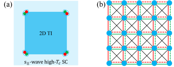
FIG. 1. Schematics of (a) a 2D TI proximitized by a nodeless high- T_c ( e.g. , Fe-based s_{\pm} -wave) superconductor yielding corner Majoranas and (b) a square-lattice model to realize (a). Details in (b) are described below Eq. (1) in the main text.
