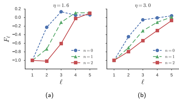
FIG. 3. Fermi liquid parameters F_{\ell} (a) slightly below the critical value of \eta for n = 2 ( \eta = 1.6 ) and (b) above the critical value of \eta for n = 2 ( \eta = 3.0 ). For larger \eta , all Fermi liquid parameters are above Pomeranchuk instability point ( F_{\ell} > -1 ) and hence the system is stable against Pomeranchuk instability in any channel. For \eta slightly below the critical value for n = 2 , only the \ell = 2 channel shows instability.
