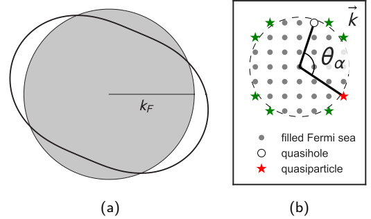
FIG. 1. (a) Deformation of the Fermi surface in the angular momentum \ell = 2 (nematic) channel. (b) Filled Fermi sea of composite fermions and a quasiparticle-quasihole pair configuration with the lowest energy marked in red. 7 other configurations with the quasihole momentum and the same kinetic energy are marked in green.
