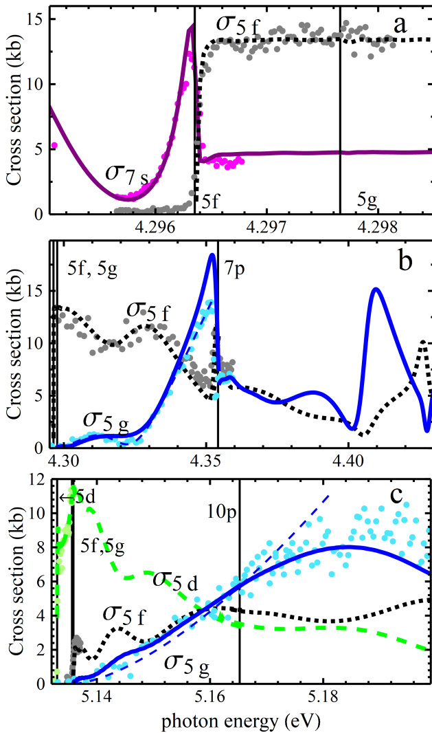
FIG. 1. Observed [21, 32, 33, 43] (round dots) and calculated PCSs for a) potassium near the 5f, 5g thresholds, b) potassium, c) sodium. PCSs for the 7s (purple curves, panel a only), 5f (black, square dots), 5g (blue, solid), and 5d (dashed green, panel c only) are shown. Thin dashed curves show TL fits.
