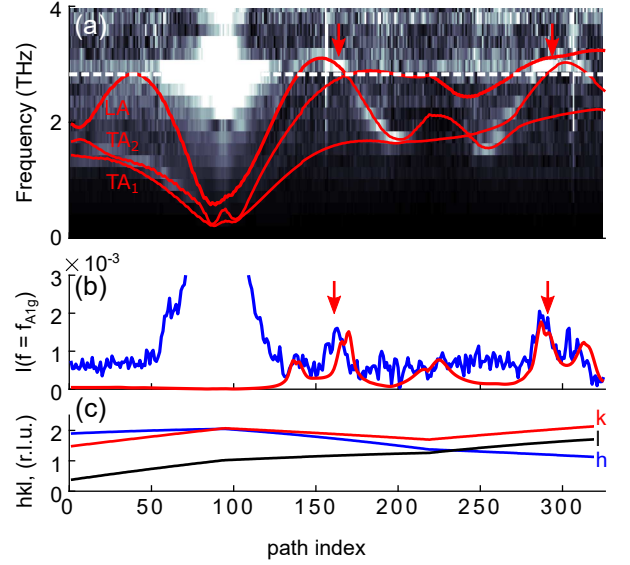
Figure 3. (a) Color online. Lineout along the cut shown in red in Fig. 2(a). The intensity is scaled by \omega^2 . The bright spot near q = 0 at 2.85 THz is from the A_{1g} mode. The second harmonic of the acoustic dispersion is plotted on top of the lineout. The A_{1g} mode frequency is represented by a white dashed line. The squeezing signal is brightest where the phonon branches intersect the A_{1g} frequency (red arrows). (b) Intensity at the 2.85 THz along the lineout shown in (a). Blue is experiment, red is the simulation as described in the text. Arrows point to the same positions along the cut as in (a). (c) The reciprocal lattice positions ( h k l ) indices (in r.l.u.) along the cut.
