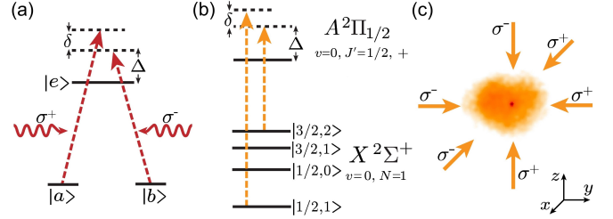
FIG. 1. (a) 3-level system exhibiting velocity-dependent dark states. Two ground states |a\rangle and |b\rangle are addressed separately by two counter-propagating laser beams. (b) Specific scheme for \Lambda -cooling of CaF. The cooling light consists of two components addressing the |J = 1/2, F = 1\rangle and |3/2, 2\rangle hyperfine manifolds. The single-photon detuning for |1/2, 1\rangle and two-photon detuning are denoted by \Delta and \delta respectively. The hyperfine spacing between |3/2, 2\rangle and |1/2, 1\rangle is h \times 73.160\ \text{MHz} [40]. (c) Schematic of \Lambda -cooling beams, overlaid with a fluorescence image of \Lambda -cooled CaF molecules. Molecules in the optical dipole trap (ODT) appear as a bright spot surrounded by a larger cloud of untrapped molecules. ( \Lambda -imaging of trapped molecules is shown in Fig. 4(c).)
