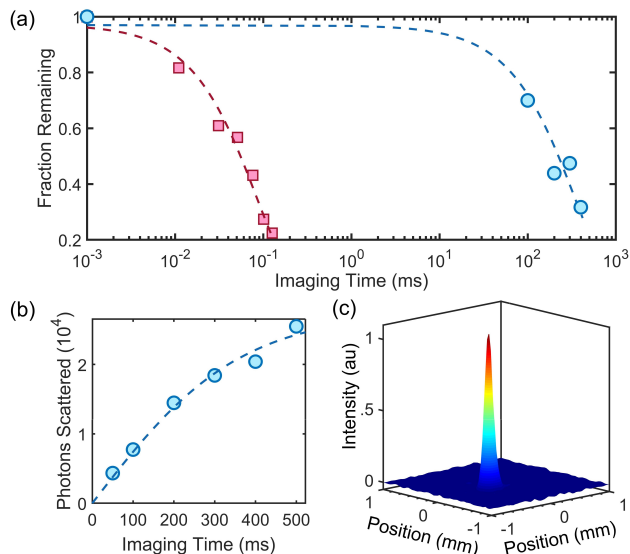
FIG. 4. (a) Fraction of molecules remaining versus imaging time for \Lambda -imaging shown (blue circles) and resonant imaging (red squares). (b) Total number of photons scattered versus imaging time (c) In-situ \Lambda -imaging of trapped molecules ( \Delta = 3.9\Gamma , \delta = 2\pi \times 90 kHz, I = 31 mW/cm 2 and R_{2,1} = 0.16 ). The exposure time is 200 ms, and 50 individual images are averaged.
