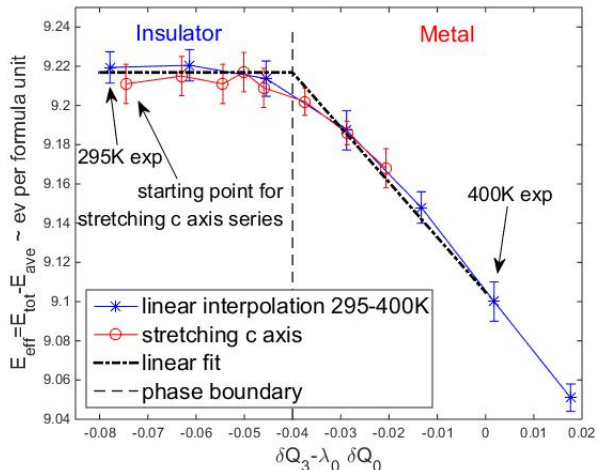
FIG. 2. Electronic energy of correlated bands E_{eff} = E_{corr} - \epsilon_{ave}N_{tot} plotted against a linear combination of octahedral parameters with \lambda_0 = 0.45 and calculated using DFT+DMFT for two series of structures: the linearly interpolated structures between the experimentally observed metallic 400K and insulating 295K structures (solid points, blue on-line) and a series obtained by starting from a relaxed insulating structure with a = b = 5.44 \text{ \AA} and stretching the c-axis (open symbols, red on-line). The bold dashed black line stands for the linear fit in eq 4 and the light dashed line shows phase boundary. The error bars are statistical errors from the Monte Carlo solution of the DMFT equations.
