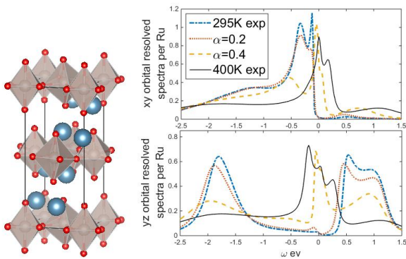
FIG. 1. Left panel: Representation of the unit cell of \text{Ca}_2\text{RuO}_4 . Gray balls are ruthenium atoms, red balls oxygen atoms and blue balls calcium atoms. Right panel: Orbitally resolved many-body densities of states for structures interpolating between experimental 295 K and 400 K structures. Upper panel: xy orbital; lower panel: yz orbital ( xz is very similar). \alpha = 0 is the 295 K structure; \alpha = 1 is the 400 K structure; \alpha = 0.4 is in the metallic phase but very close to the transition point; the \alpha = 0.6, 0.8 spectra are very similar to the 400 K spectra and are omitted for clarity.
