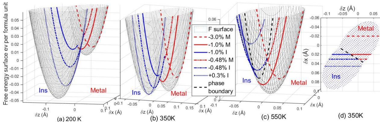
FIG. 3. Free energy surfaces computed for unconstrained bulk \text{Ca}_2\text{RuO}_4 at temperatures 200 K(a), 350 K(b), and 550 K(c), along with projection of 350K surface onto x-z plane (d). The black dashed line in panels (c) and (d) shows the metal-insulator phase boundary. The solid and dashed lines show the structural trajectories which the system can explore for films grown under the epitaxial strain conditions given in the legends. The blue and red regions of the lines indicate insulating and metallic regions respectively.
