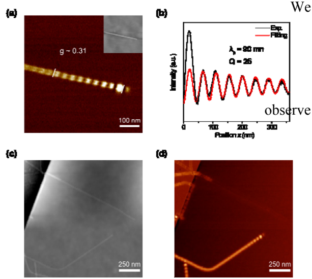
FIG. 2. Near-field optical nanoscopy characterizations on SWNTs on hBN. (a) Near-field optical nanoscopy image of an individual metallic SWNT with a diameter of \sim 1 nm. Inset shows the corresponding topography image that is simultaneously recorded. (b) Experimental intensity profile (in black) of Luttinger liquid plasmon oscillations and the corresponding theoretical fitting (in red) with the damped oscillator form e^{-2\pi x / (Q \cdot \lambda_p)} \sin((4\pi x) / \lambda_p) along the tube axis between two bars in (a), where \lambda_p is the plasmon wavelength and Q is the quality factor. Luttinger parameter g \sim 0.31 (shown in (a)) is directly obtained from the measured plasmon wavelength \lambda_p . (c) AFM topography image of an individual metallic SWNT (tube A) and an individual semiconducting SWNT (tube B) on hBN with similar diameters \sim 0.8 nm. (d) The corresponding near-field optical nanoscopy image of (c). The metallic SWNT (tube A) exhibits prominent Luttinger liquid plasmon oscillations, whereas the semiconducting SWNT (tube B) barely shows any near-field optical response owing to the finite bandgap.
