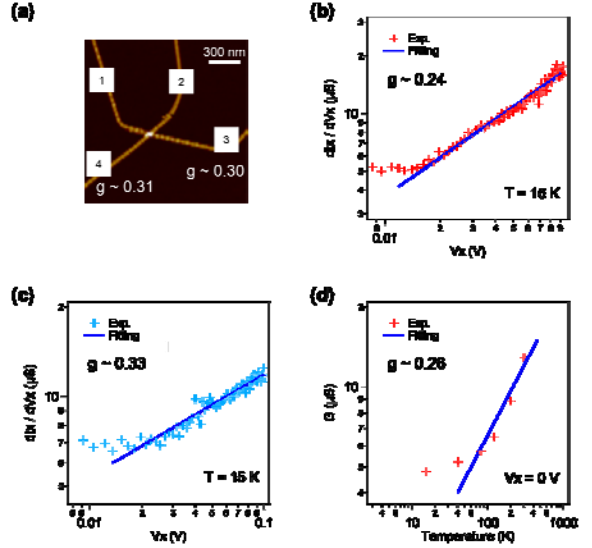
FIG. 4. Correlation of electron tunneling and plasmon propagation in Luttinger liquid (device #3). (a) Near-field optical nanoscopy characterization on a metallic SWNT cross junction. Luttinger parameters are determined to be g \sim 0.30 (tube 1-3) and g \sim 0.31 (tube 2-4), respectively. Metal contacts are denoted by numbers. (b) Differential conductance ( dI_x/dV_x ) measurement of the electron tunneling probability across the Luttinger liquid junction as a function of voltage drop across the junction ( V_x ) at 15 K. Measurements are carried out in a four probe configuration where the electrical current is forced to flow through contacts 1 and 2 and voltage drop is measured through contacts 3 and 4. A power function fitting (blue line) yields g \sim 0.24 by using Eq. (1). (c) dI_x/dV_x at 15 K at a different backgate voltage with respect to (b), which yields g \sim 0.33 . (d) The corresponding temperature-dependent electron tunneling data (zero V_x ) with the same backgate voltage as in (b), which yields a best fit of g \sim 0.26 .
