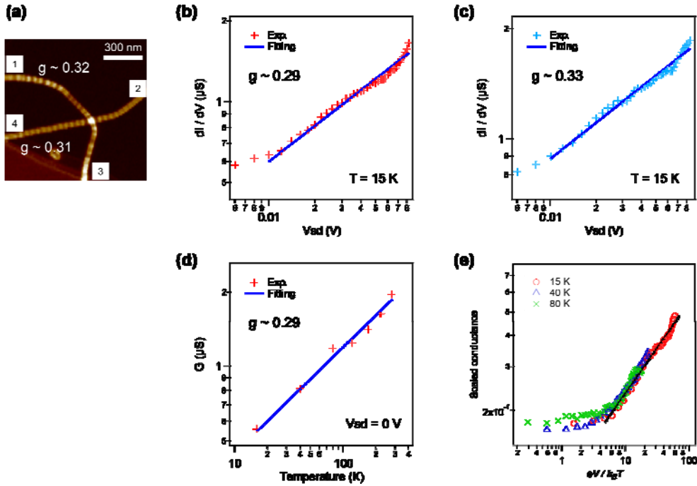
FIG. 3. Correlation of electron tunneling and plasmon propagation in a Luttinger liquid (device #1). (a) Near-field optical nanoscopy characterization on a metallic SWNT cross junction. Luttinger parameters are determined to be g \sim 0.32 (tube 1-3) and g \sim 0.31 (tube 2-4) for each of two nanotubes from the measured Luttinger liquid plasmons. Metal contacts are denoted by numbers. (b) dI/dV measurement of the electron tunneling probability across the Luttinger liquid junction as a function of electrical bias ( V_{sd} ) at 15 K (through contacts 1 and 4). The SWNT junction dominates the total resistance and a two probe measurement is carried out. A power function fitting (blue line) yields the power index \alpha \sim 0.43 which corresponds to g \sim 0.29 by using Eq. (1). (c) Power-law scaling behavior on electrical bias at 15 K at a different backgate voltage with respect to (b), which yields g \sim 0.33 . (d) The corresponding temperature-dependent electron tunneling data (zero V_{sd} ) with the same backgate voltage as in (b), which yields g \sim 0.29 . (e) Scaled conductance (dI/dV)/T^\alpha as a function of eV/k_B T at different temperatures, where \alpha is the power component with bias scaling at each temperature. All data collapse onto a single curve reasonably well, which provides an independent verification of Luttinger liquid behavior.
