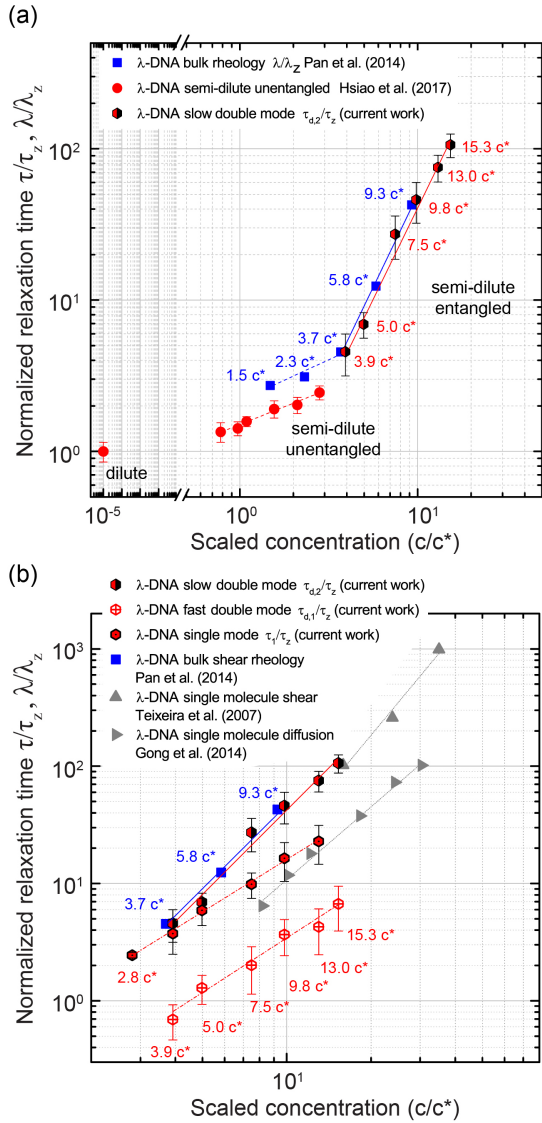
FIG. 3. Normalized longest relaxation times \tau/\tau_z and \lambda/\lambda_z as a function of scaled polymer concentration c/c^* . (a) Power-law relaxation time scaling behavior across the semi-dilute unentangled and entangled regimes. (b) Characteristic longest relaxation times in the entangled regime.
