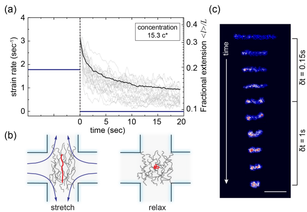
FIG. 1. Single molecule studies of polymer relaxation in entangled DNA solutions. (a) Flow deformation protocol and polymer relaxation process. At time t = 0 , the flow is stopped and chains relax to equilibrium. Single molecule trajectories (grey) and ensemble averaged fractional extension (black) at 15.3 c^* . (b) Schematic of experiment showing a single fluorescently labeled tracer \lambda -DNA molecule (red) in a background of entangled DNA solution. (c) Snapshots of a single tracer DNA molecule relaxing in an entangled solution, showing double-mode relaxation behavior. Scale bar: 5 \mu\text{m} ; \delta t is time between images.
