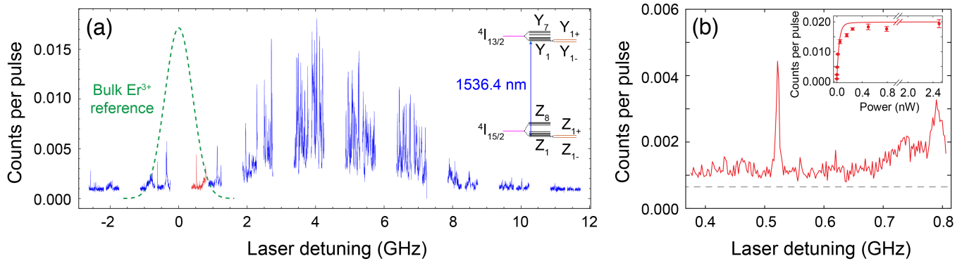
FIG. 2. Photoluminescence excitation (PLE) spectrum of single ions in a dilute \text{Er}^{3+} ensemble. (a) PLE spectrum, measured by scanning the laser frequency and cavity resonance (with linewidth \kappa = 2\pi \times 3.85 GHz) together through a spectral region near the bulk Er:YSO absorption resonance at 1536.46 nm (determined from a second crystal, and indicated schematically by the green dashed line). The vertical axis indicates the average number of photons detected in an 82 \mu\text{s} integration window following each excitation pulse (as in Fig. 1d). The spectrum shows individually resolvable peaks, which we interpret as the optical transitions of single \text{Er}^{3+} ions. The interruptions in the scan result from spectral regions that are inaccessible with our laser stabilization technique. Inset: Energy levels of \text{Er}^{3+} in YSO. The crystal field splits the ^{2S+1}L_J states of the free \text{Er}^{3+} ion (magenta lines) into J + 1/2 Kramers doublets (black lines), which further split into single states in a magnetic field (orange lines). The cavity is resonant with the Z_1 - Y_1 transition at 1536.46 nm (YSO site 1). (b) Expanded view of the red portion of (a), showing an isolated line with a width of 5 MHz (full-width at half-maximum, FWHM) on a nearly dark-count-limited background (gray dashed line), characteristic of the tails of the inhomogeneous distribution. Inset: The background-subtracted height of this isolated peak saturates with increasing excitation power. The solid line is a model based on independently measured parameters [33].
