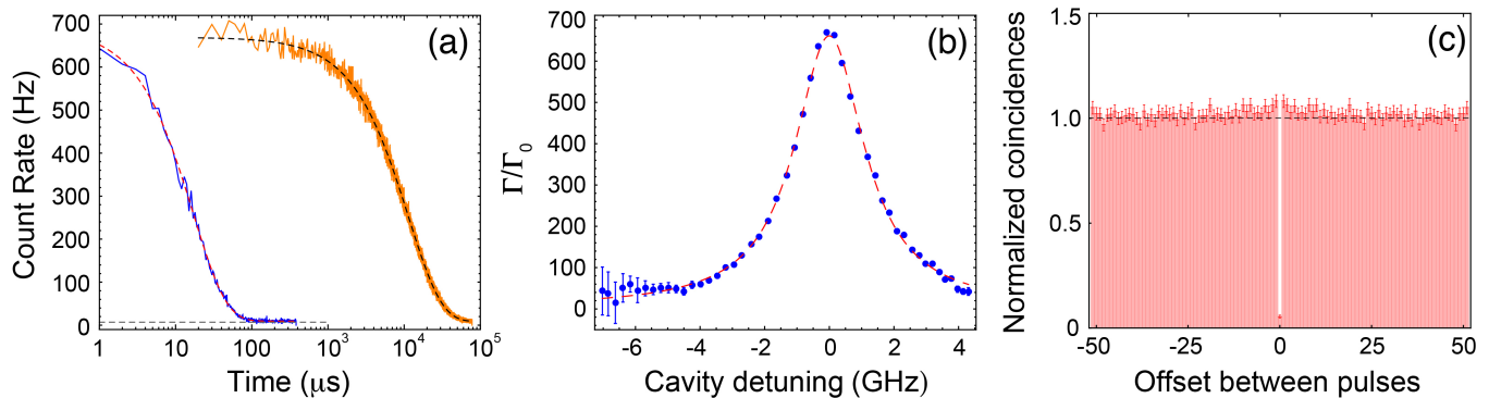
FIG. 3. Quantifying the \text{Er}^{3+} -cavity coupling, and measurement of g^{(2)} . (a) Time-resolved fluorescence from a single cavity-coupled \text{Er}^{3+} ion (blue) following an excitation pulse, which decays to the detector dark count rate (gray dashed line). The fluorescence from a bulk ensemble without cavity enhancement is shown for comparison (orange; measured in a second crystal, and on an arbitrary vertical scale). (b) Fixing the laser frequency to the atomic transition and sweeping the cavity resonance reveals that the decay rate enhancement \Gamma/\Gamma_0 varies with the atom-cavity detuning. A Lorentzian fit to the data (red dashed curve) yields a width of 2.62 \pm 0.04 GHz (in agreement with the cavity linewidth), and a maximum decay rate enhancement of P = 658 \pm 5 . (c) Second-order autocorrelation function ( g^{(2)} ) of the fluorescence from a single ion. We bin all photons detected after a single excitation pulse into a single time bin, so the horizontal axis shows the autocorrelation offset in units of the pulse repetition period ( 100 \mu\text{s} ). The data is symmetric around zero offset since a single detector is used to record the fluorescence and compute a true autocorrelation; however, both positive and negative offsets are plotted for clarity.
