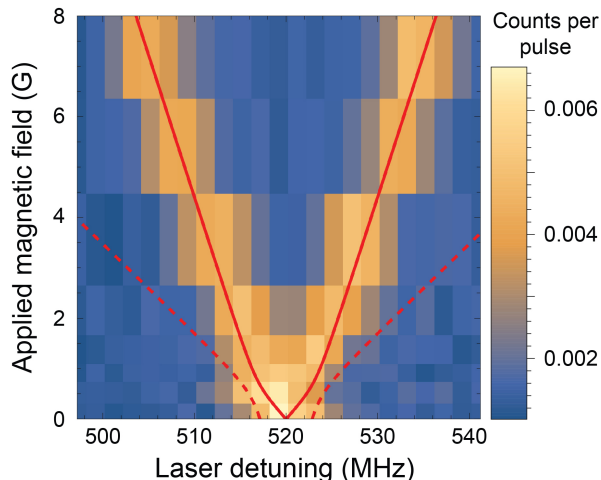
FIG. 4. Zeeman splitting of a single \text{Er}^{3+} ion spectral line. A magnetic field splits a single spectral line into two transitions. The field is oriented approximately 45 degrees between the D_1 and D_2 axes in the D_1 - D_2 plane. The predicted transition frequencies are shown with red lines, including an offset field of around 1 G. Since the g -factors are highly anisotropic, the slope of the predicted splitting is not linear when the applied field is smaller in magnitude than the offset field, which has a different orientation.
