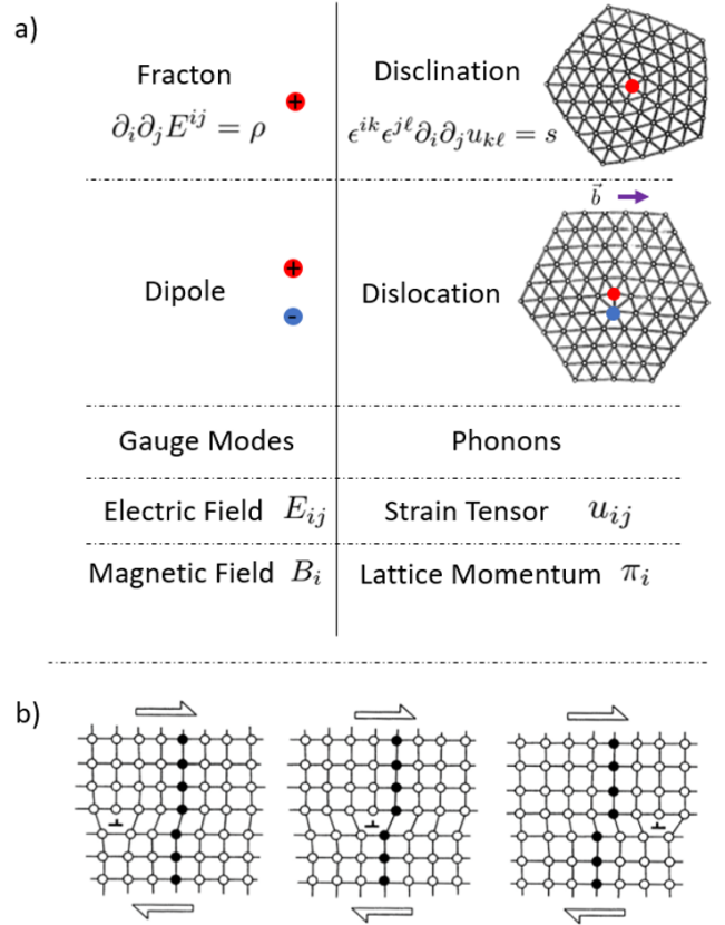
FIG. 1: a) The Fracton-Elasticity Dictionary: Excitations and operators of the scalar-charge tensor-gauge theory are in one-to-one correspondence with those of a two-dimensional quantum crystal. (Pictures of lattice defects adapted from Ref. 33.) b) A dislocation can only freely move by gliding along its Burgers vector \vec{b} , while dislocation climb (motion perpendicular to \vec{b} ) requires the presence of vacancy/interstitial defects.
