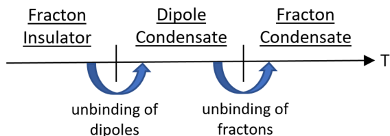
FIG. 2: The duality with elasticity theory predicts that the fracton gauge theory exhibits two finite-temperature phase transitions, corresponding to unbinding of dipoles and fractons, respectively.
